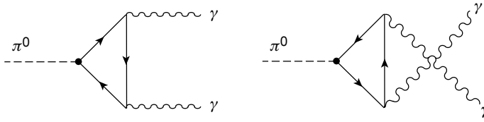
Fig. 3.6. \pi^0 \rightarrow \gamma\gamma decay from the quark triangle.
