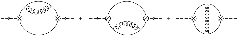
Fig. 11.3. Two-loop perturbative contribution to the pseudoscalar two-point function.
