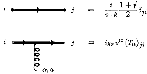
Fig. 44.2. Feynman rules of the HQET ( i, j and a are colour indices). A heavy quark with velocity v is represented by a double line. The residual momentum k is defined in Eq. (44.2).
