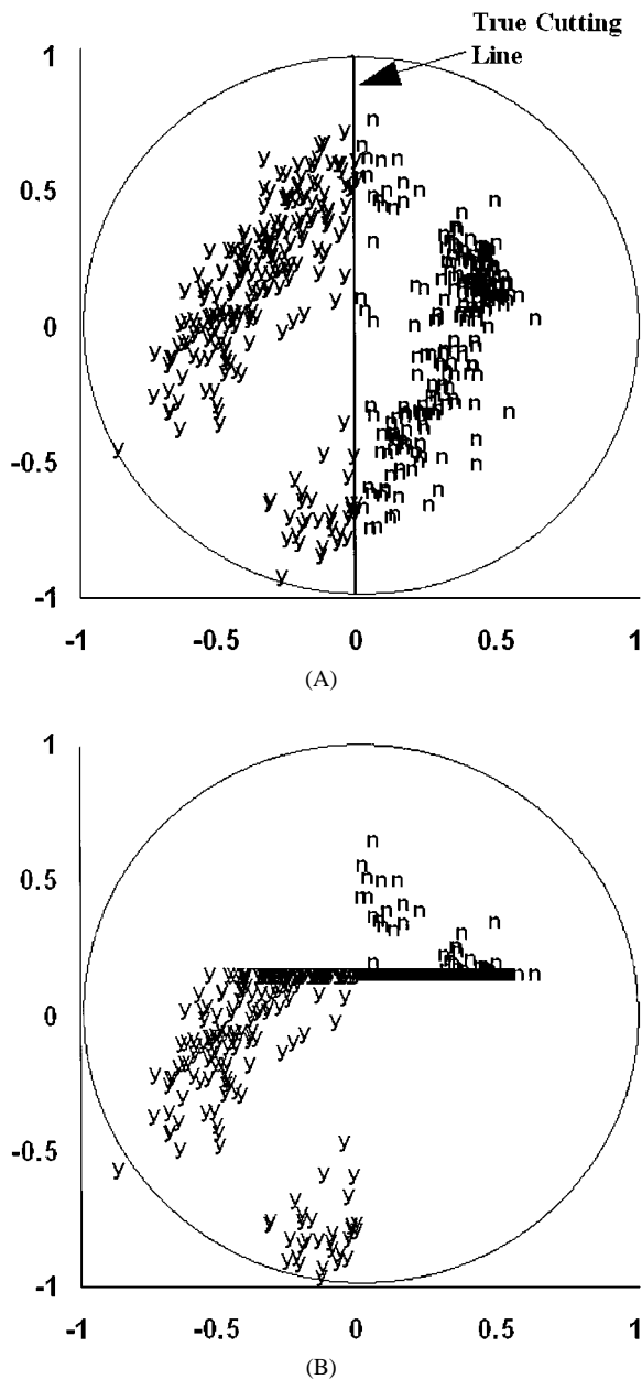
Fig. 3 (A) True cutting line. (B) Initial estimate of cutting plane.
