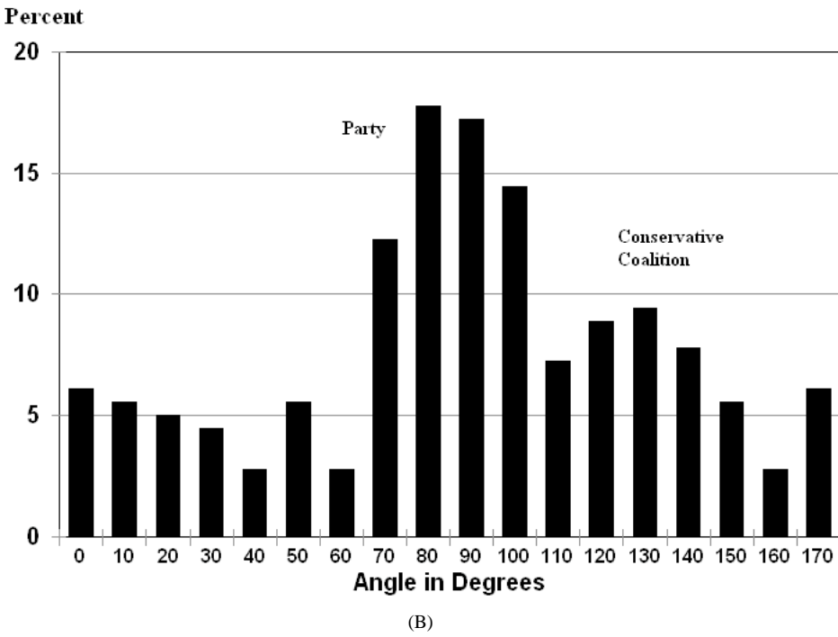
Fig. 5 (A) Senator locations. D, Northern Democrat; S, Southern Democrat; R, Republican. (B) Eighty-fifth Senate, 1957–1958: cutting line angles.
