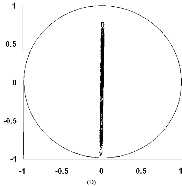
Fig. 3 (Continued) (C) Second estimate of cutting plane. (D) Thirty-fifth estimate of cutting plane.
