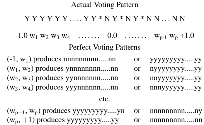
Fig. 2 Calculating the correct classification.
