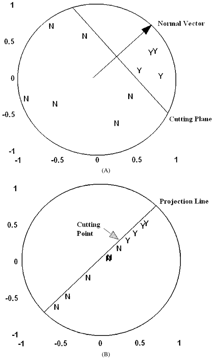
Fig. 1 (A) Original positions in two dimensions. (B) Points projected onto line.
