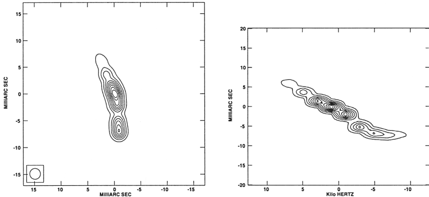
Figure 3. Left: a super-resolution image of the L1206 feature A, all spectral channels are averaged together. Contours are 0.13 \times (1, 2, 3, 4, 5, 6, 7, 8, 9) Jy/beam. Right: declination – frequency diagram for the left image. Contours are 0.43 \times (1, 2, 3, 4, 5, 6, 7, 8, 9) Jy/beam.
