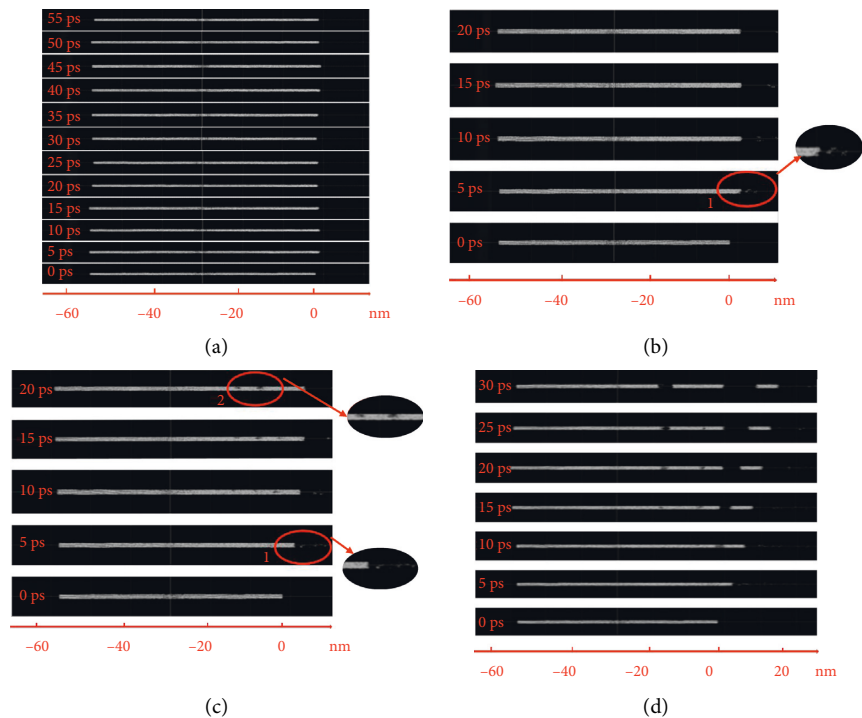
FIGURE 4: Schematic diagram of atomic snapshots at different energy flux: (a) 1000 J/m 2 , (b) 2232 J/m 2 , (c) 3188 J/m 2 , and (d) 4782 J/m 2 .
