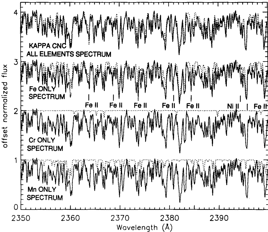
FIGURE 2: A NOVEL APPROACH TO IDENTIFYING LINE BLENDS. Vertical offsets by addition of 0, 1, 2, or 3 used. Solid lines show the IUE co-added observation of \kappa Cnc; dotted lines show synthetic spectra. The synthetic spectrum labeled "All Elements Spectrum" is calculated with all elements using optical abundances. The "Fe Only Spectrum" is a synthetic spectrum showing only the Fe lines (see text). Similar single-element spectra were calculated for Cr, Mn (both shown here), Ni, Co, and Ti from 1150 to 3000Å.
