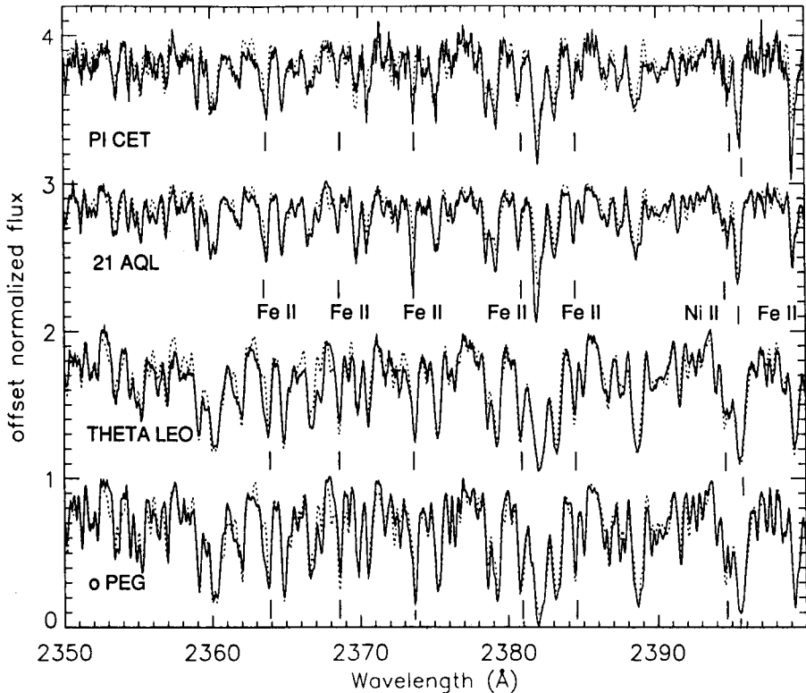
FIGURE 1: SAMPLE OF CONTINUUM FITS IN FOUR STARS. Each star is vertically offset by addition of 0, 1, 2, or 3 to the normalized flux. The solid lines show the IUE co-added observations; dotted lines show synthetic spectra (based on optical abundances) used for modelling the continuum. Lines used in our abundance analyses are denoted by vertical bars. Note the general agreement between initial optical-based models and observations. Also note that a single Fe abundance will not fit each Fe II line in a given star.
