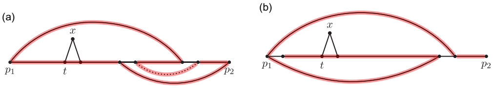
The vertex right to the neighbour of p_1 is adjacent to the vertex to the right of the neighbour of p_2 .
