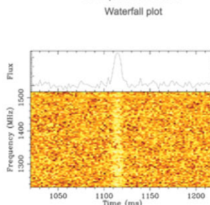
Frequency vs. time waterfall plot for FRB010125 dedispersed to the optimal DM. Not bandpass corrected.
