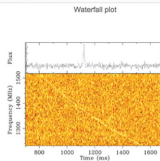
Frequency vs time waterfall plot for FRB010125. Not bandpass corrected.
