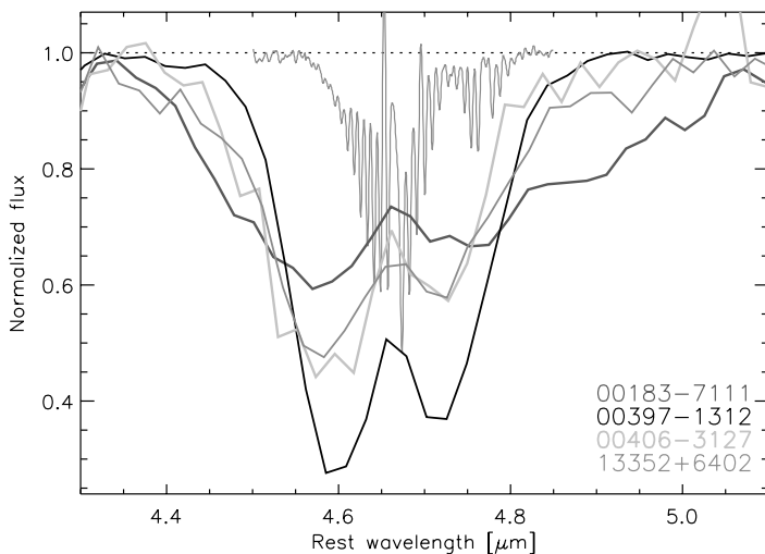
Figure 7. Comparison of the normalized flux profiles for the CO absorption features in the spectra of Sgr A* ( dark grey narrow profile; Moneti et al. 2001) and the four ULIRGs shown in Figure 6. Individual lines are resolved in the high-resolution ISO-SWS spectrum of Sgr A*.
