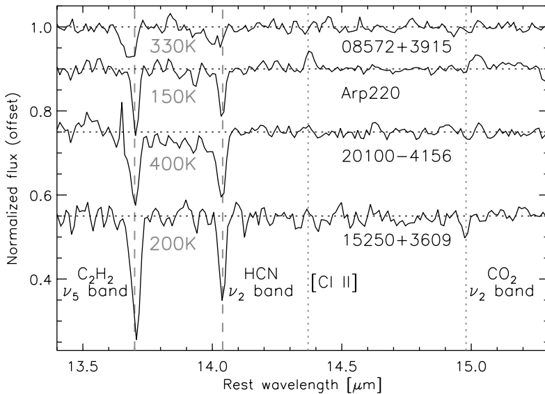
Figure 5. Continuum-normalized high-resolution IRS spectra of four deeply obscured ULIRGs. The spectra reveal the presence of gas absorption bands of \text{C}_2\text{H}_2 at 13.7\ \mu\text{m} , HCN at 14.03\ \mu\text{m} and \text{CO}_2 at 15.0\ \mu\text{m} . Best fitting excitation temperatures for the \text{C}_2\text{H}_2 and HCN absorption bands are indicated on the plot. Also indicated is the [Cl II] line at 14.37\ \mu\text{m} in Arp 220.
