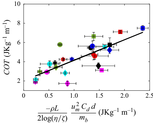
Figure 29. Experimentally obtained COT (3.28) values plotted versus the analytically predicted values given by (3.30) and data point legends are given in figure 14. The black line shows linear fit with R^2 = 0.59 .
