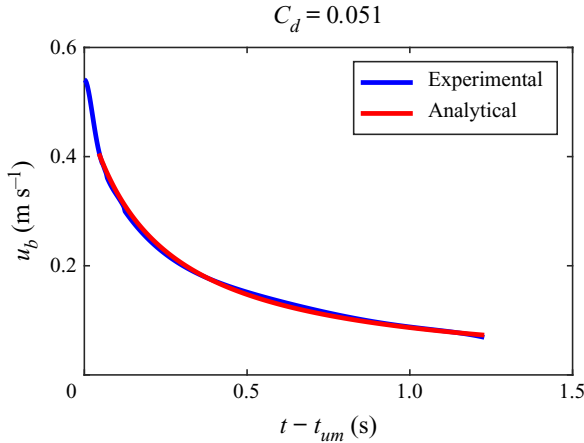
Figure 16. The translational velocity of the body in the retardation phase for the case with d^* = 1.0 , Kt = Kt_1 , M^* = 1.0 and 2\theta_o = 45^\circ . Blue curve represents a fit to the experimental data, and the red curve is data obtained using (3.12); \phi = 9.5 for this case.
