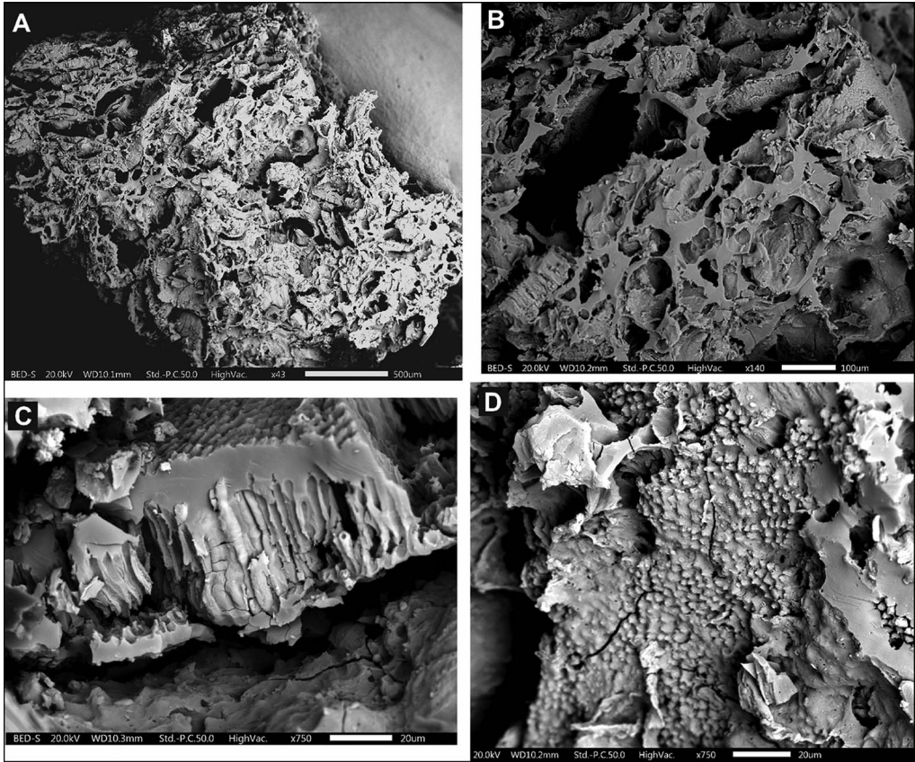
Figure 2. Pulse-rich charred plant food fragment from Franchthi Cave (context no. H1A 168, Final Palaeolithic, Epigravettian): A) overview; B–D) close-ups of pulse seed fragments and seed coat remains (SEM micrographs taken by C. Kabukcu).
