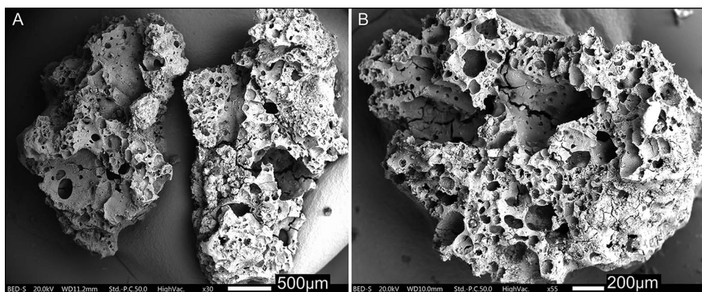
Figure 4. Charred plant food remains from Franchthi Cave, with a homogenised matrix (context no. H1A 172, Upper Palaeolithic, Mediterranean Gravettian): A) overview; B) close-up showing variable sizes of voids (SEM micrographs taken by C. Kabukcu).
