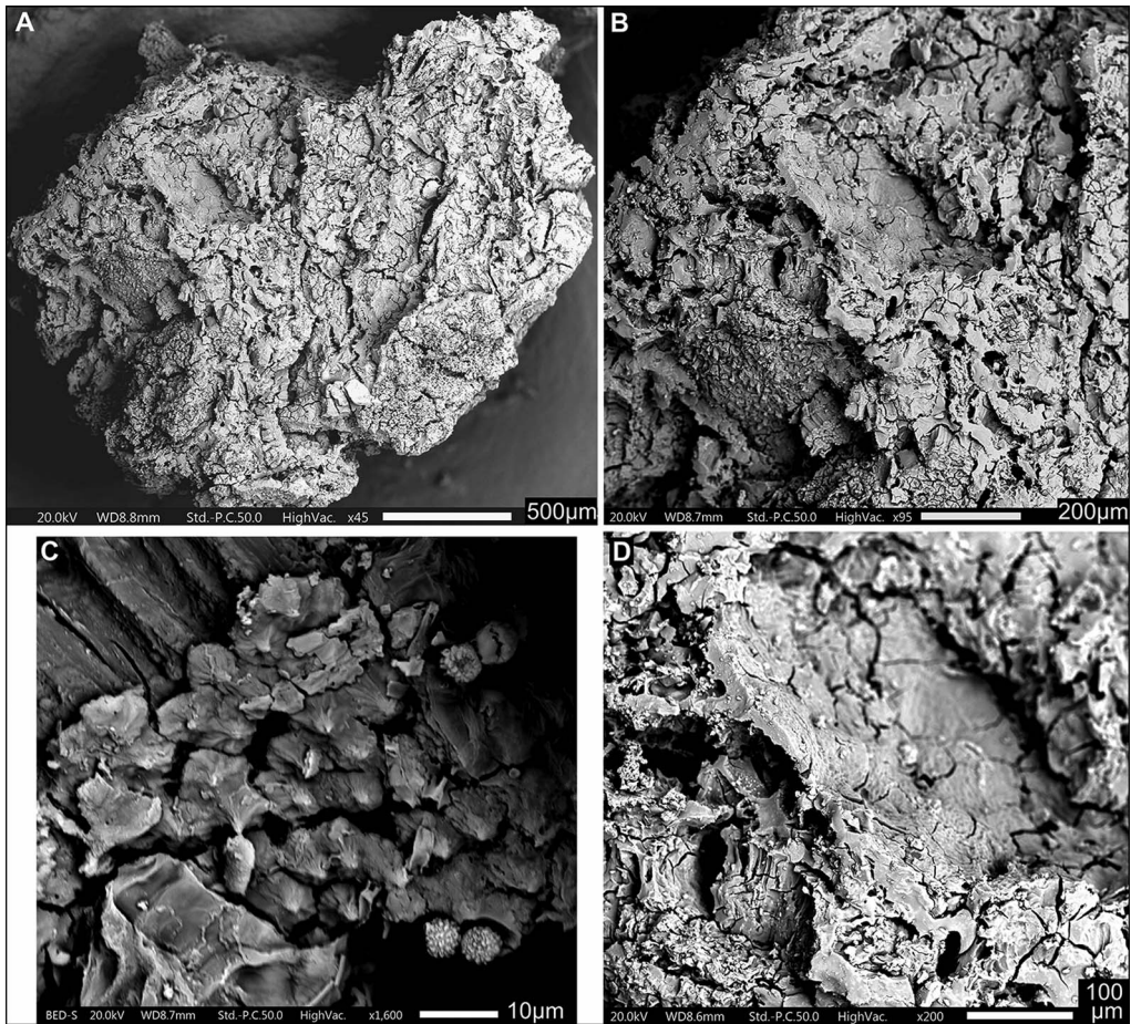
Figure 8. Charred plant food remains from Shanidar Cave (context no. 1866, Upper Palaeolithic, Initial Baradostian): A) overview; B) & D) close-up of cf. Pistacia nutshell/periocarp remain; C) close-up of pulse seed coat pattern (Fabaceae) (SEM micrographs taken by C. Kabukcu).
