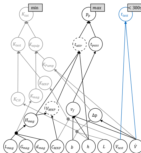
Figure 7. Adapted ADG due to the changed QoI detectability to p_p
