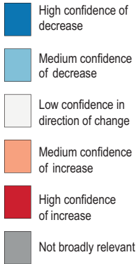
(a) Summary of confidence in direction of projected change in climatic impact-driver (CID) (WGI AR6, 2021, Tables 12.3 to 12.9)
