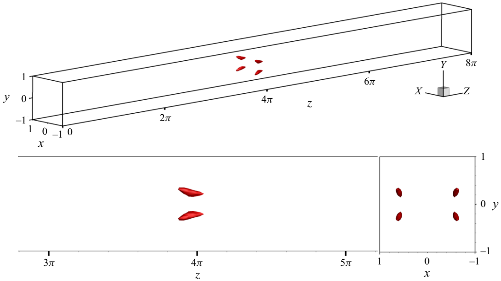
Figure 3. Identified invariant state visualised by contours of the second invariant of the velocity gradient tensor normalised by w_b , taken at Q/w_b^2 = 1.5 \times 10^{-1} .
