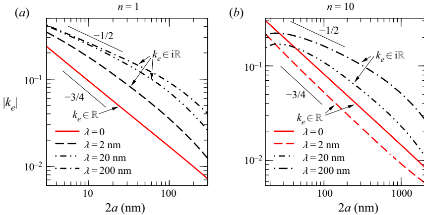
Figure 11. Absolute value of the effective aspect ratio k_e versus the platelet length 2a for \xi = 0.25 nm and for n = 1 (a) and n = 10 (b). The black lines correspond to the purely imaginary values of k_e and the red lines to real values of k_e .
