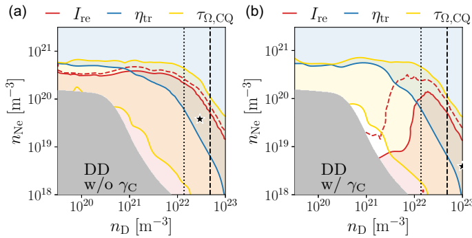
FIGURE 3. Regions of safe operation (shaded) with regards to I_{re} (red), \eta_{tr} (blue) and \tau_{\Omega, CQ} (yellow) for D operation (a) without Compton generation and (b) with Compton generation. Additionally, the red dashed line indicates where the runaway current is 1 MA, bounding the tolerable region of operation. The optimal sample is indicated by a star, the upper design limit of the D density during MGI in SPARC is indicated by the dashed vertical line for 44 % assimilation ( n_D = 4.8 \times 10^{22} \text{ m}^{-3} ) and the dotted vertical line for 10 % assimilation. The grey area covers the region of incomplete TQ.
