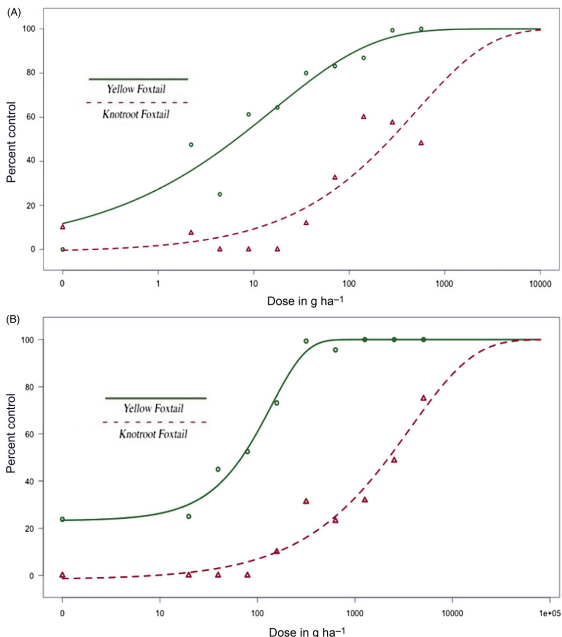
Figure 1. Percent visible injury to the nontreated control of yellow and knotroot foxtail 28 d after application with increasing rates of pinoxaden (A) and sethoxydim (B). The regression parameter is determined by the Weibull model with four parameters: f(x) = C + (D - C) \times \exp[-\exp[b(\log x - \log e)]] . Each bullet represents the average control for each treatment.
