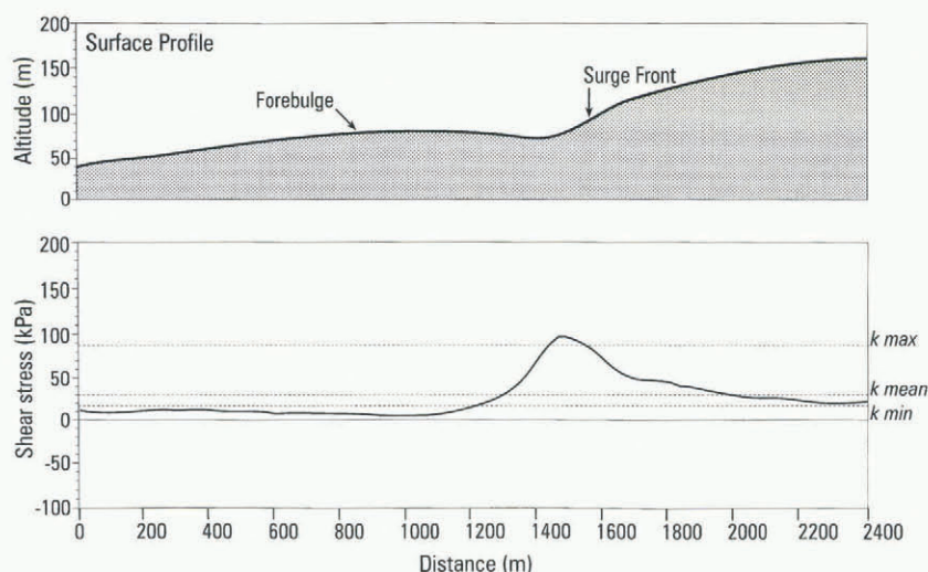
Fig. 4. 1995 surface profile of Bakaninbreen, showing basal shear stress calculated from Equation (2). Maximum, minimum and mean basal sediment yield strengths calculated from Equation (1) are shown as horizontal dashed lines. Minimum basal sediment yield strength is consistently exceeded up-glacier of the surge front. Basal sediments in this region are therefore likely to be deforming.
