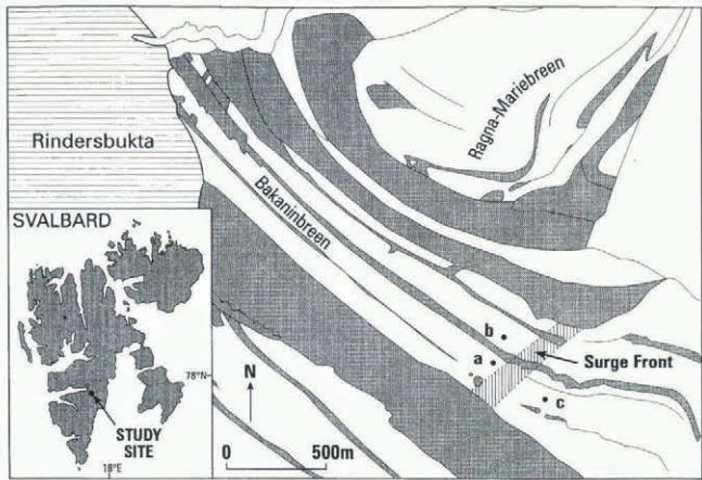
Fig. 1. Map of Bakaninbreen, Svalbard, showing location of surge front in 1995 (cross-hatched) and position of ploughmeter placements: (a) PL-2, (b) PL-3, and (c) PL-5.
