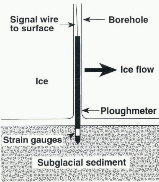
Fig. 2. Schematic diagram showing a ploughmeter installed at the glacier bed. The ploughmeter is hammered into basal sediments such that the upper part becomes trapped within glacier ice. Strain gauges bonded to the immersed section respond to elastic bending of the ploughmeter as the device is dragged through basal sediments by the motion of the glacier.
