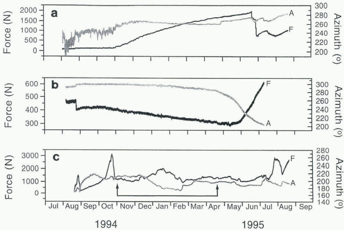
Fig. 3. Long-term force and azimuth records from ploughmeters: (a) PL-2, (b) PL-3 situated down-glacier of the surge front, and (c) PL-5 situated up-glacier of the surge front. Force and azimuth are labelled F and A, respectively. Note the steadily increasing force trace after October 1994 (PL-2) and May 1995 (PL-3). Ploughmeter PL-5 shows a more jagged force trace, consistent with ploughmeter motion through an area of coarse-grained bed. Arrows on (c) PL-5 indicate period over which yield-strength calculations have been made.
