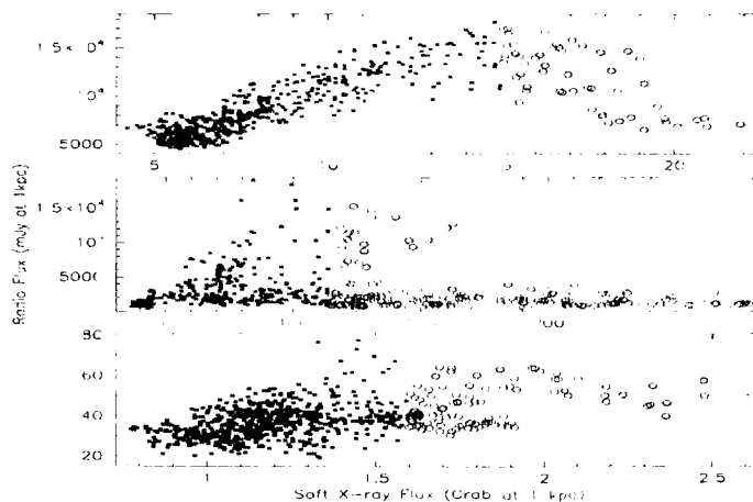
Fig. 1. Scatter diagram of soft X-ray emission and radio emission of Cygnus X-3 (top panel, GRS 1915+105 (middle panel) & Cygnus X-1 (bottom panel), in the low as well as hard state, after removing the radio flares.
