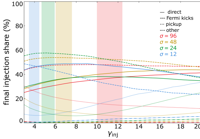
FIGURE 13. Injection shares at t = t_{\text{onset}} + 3 L_x/c as a function of \gamma_{\text{inj}} for 2-D simulations. The solid bars indicate the error about the measured injection energies.
