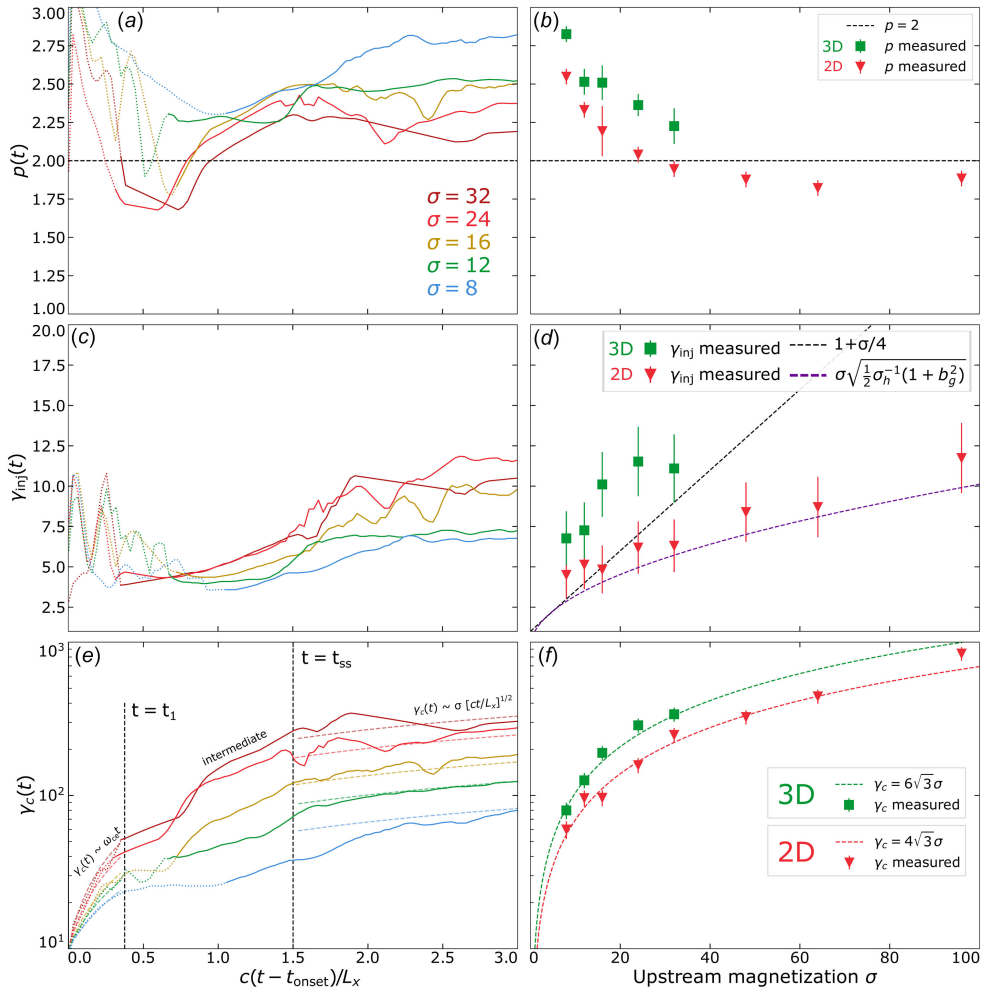
FIGURE 5. Spectral parameters measured via fitting procedure (described in Appendix B ) for various \sigma at each time step for 3-D simulations ( a , c , e ) and at t = t_{\text{onset}} + 3 L_x/c for all simulations ( b , d , f ). Dotted coloured lines in ( a , c , e ) indicate time steps where the power-law extent is short, i.e. \gamma_c/\gamma_{\text{inj}} < 10 . In ( b , d , f ), red triangles are 2-D runs and green squares are 3-D runs. ( a , b ) Power-law indices p(t) and p(t_{\text{onset}} + 3 L_x/c) . ( c , d ): Injection energies \gamma_{\text{inj}}(t) and \gamma_{\text{inj}}(t_{\text{onset}} + 3 L_x/c) . The dashed black line in ( d ) shows linear scaling, assuming \gamma_{\text{inj}} = 1 + \sigma/4 and the dashed purple line shows \gamma_{\text{inj}} \simeq \sigma [\sigma_h^{-1} (1 + b_g^2)/2]^{1/2} (i.e. (2.7)), derived in § 2.1. ( e , f ) High-energy cutoffs \gamma_c(t) and \gamma_c(t_{\text{onset}} + 3 L_x/c) . The semi-transparent dashed coloured lines in ( e ) show the fit from (4.2) and the green (red) dashed line in ( f ) shows it evaluated at t_{\text{onset}} + 3 L_x/c , i.e. \gamma_c(\sigma) = 6\sqrt{3}\sigma in three dimensions ( \gamma_c(\sigma) = 4\sqrt{3}\sigma in two dimensions).
