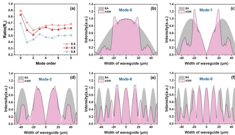
Figure 4. (a) Energy retained after transmitting different lateral modes through ASW structure with microstructure size ratio of 0.4, 0.5, and 0.6. (b)-(f) Simulated optical field distribution of modes with order numbers m=0, 1, 3, 6, and 8 at the facet of conventional BA lasers and ASW lasers with microstructure size ratio of 0.5.
