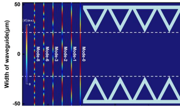
Figure 2. Details of the TSC structure. The inset shows the near-field distribution of different order modes of conventional BA lasers.
