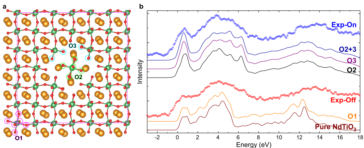
Figure 2. (a) c_t axis-projected defect supercell (supercell boundary is presented by the pink box) for DFT calculation, where each position of O of interest are indicated. (b) Experimental O K core-loss EELS fine structures and calculated O partial-DOS; “Exp-On” and “Exp-Off” represent experimental EELS on and off the defect and the calculated partial-DOS for the O positions in (a) are accordingly labeled. The calculated O partial-DOS for pure NdTiO 3 is also presented.
