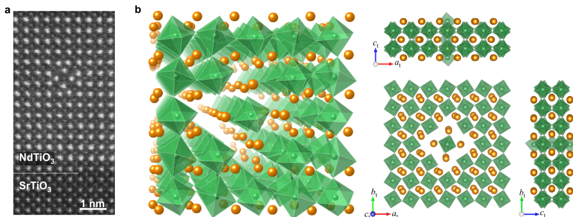
Figure 1. (a) HAADF-STEM image of a line defect in a NTO film on a STO substrate, where the NTO film is viewed along the c_t axis. (b) Perspective atomic model for the defect and its a_t , b_t , and c_t axis projections. Yellow spheres are Nd and green octahedrons represent Ti coordinated by six O.
