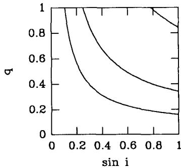
FIGURE 2. Contours of constant mass function in the mass-ratio - \sin i plane.
