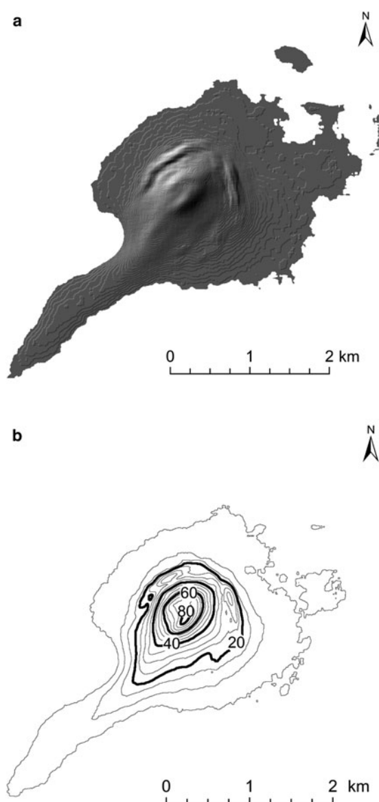
Fig. 8. (a) A hillshade of the difference between the adjusted 1998 SAR DEM and the 2010 lidar DEM. (b) A contour map of the inferred depth of the subglacial water body emptied in the 2010 flood, contour interval of 5 m. The data are smoothed with a 100 \text{ m} \times 100 \text{ m} window.
