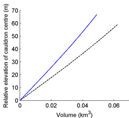
Fig. 5. Hypsometric curves for the subglacial lake below the western Skaftá cauldron showing lake volume as a function of the elevation of the cauldron centre. The result of the Elmer/Ice modelling (dashed curve) and a scaled curve that fits the observed flood volume vs. ice-shelf lowering in the September/October 2006 jökulhlaup (solid curve) are shown.
