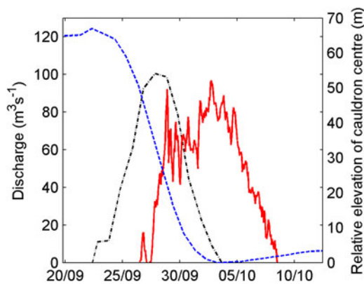
Fig. 6. Back-calculated discharge of jökulhlaup water (solid curve) at the glacier terminus during the jökulhlaup in September/October 2006 after subtracting base flow from the glacier and tributary rivers upstream of the Sveinstindur hydrometric station. The relative elevation of the cauldron centre, as measured with GPS, is also shown (dashed curve) as well as the calculated outflow from the subglacial lake (dash-dotted curve) derived from the lowering of the ice surface elevation using the hypsometric curve for the subglacial lake.
