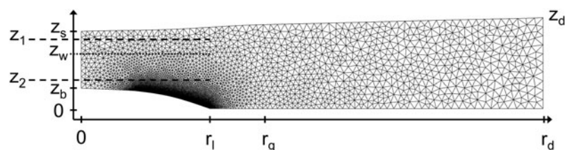
Fig. 4. The Elmer/Ice computational finite-element mesh for the cylindrically symmetric model of a glacier on a flat bed overlying a subglacial lake with dimensions corresponding to the western Skaftá cauldron. The figure explains the notation used to define the geometry of the model: the elevation of the ice surface, z_s , and the bottom of the ice, z_b , the time-dependent piezometric water level of the subglacial water lake, z_w , the radial distance to the grounding line, r_l , the radius of the geothermal area, r_g , the radius to the ice divide at the boundary of the cauldron ice flow basin with the surrounding ice cap, r_d and the ice-surface elevation at the ice divide, z_d . A jökulhlaup is released when z_w reaches a critical level z_1 and terminated when z_w reaches z_2 .
