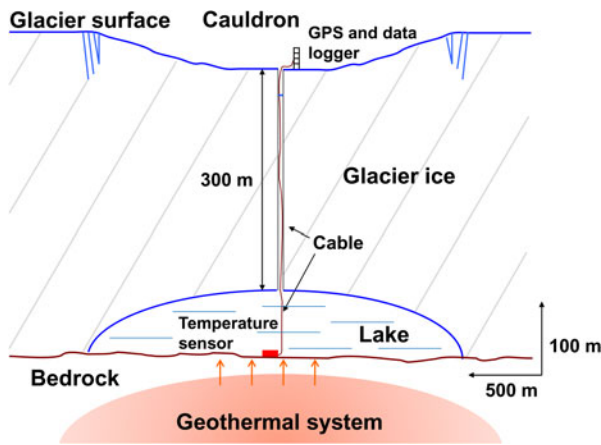
Fig. 3. Schematic drawing of the western Skaftá cauldron showing the ~300 m thick floating ice shelf penetrated by a drillhole into the ~100 m deep subglacial lake and the scientific instruments deployed in the lake and on the glacier surface in the campaign in 2006. Note that the vertical scale is exaggerated five-fold.
