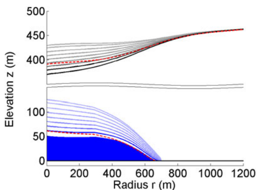
Fig. 7. Lake and surface geometry during a jökulhlaup modelled with Elmer/Ice. The geometry is drawn at daily intervals with darker colour as time progresses. The lake and surface geometries 1 month after the end of the jökulhlaup are also drawn (dashed curves).
