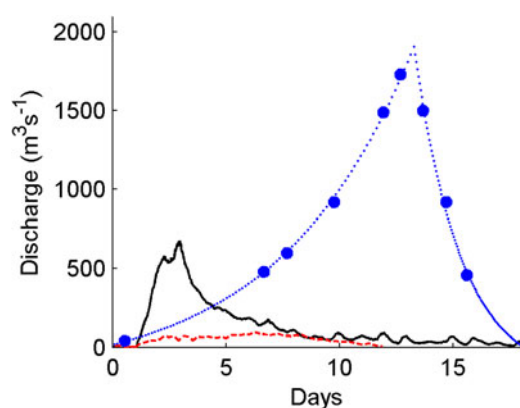
Fig. 2. Comparison of the hydrographs of a large rapidly rising jökulhlaup in 2002 (solid curve) and the small jökulhlaup in 2006 with a rapid initial rise, which is the subject of this paper (dashed curve), both from the western Skaftá cauldron. The hydrograph of a typical slowly rising jökulhlaup from Grímsvötn in 1986 (dotted curve) is also shown. The hydrograph of the Grímsvötn jökulhlaup is based on discrete discharge measurements which are shown as dots. The rapid rise of the hydrograph of the 2006 jökulhlaup is more clearly visible in Figure 6 which shows the same discharge curve with the vertical scale expanded.
