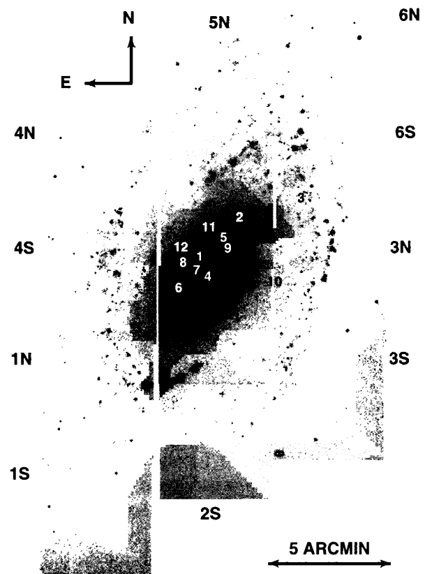
Fig. 1. Spatial distribution of novae in M81
