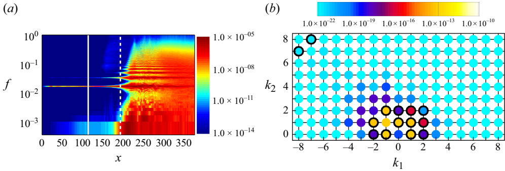
Figure 17. Streaky wave family: power spectra of the wall pressure fluctuations (a) and wavenumber bispectrum (b) for sensor G_3 located at the separation point, denoted by the white solid vertical lines on plot (a).
