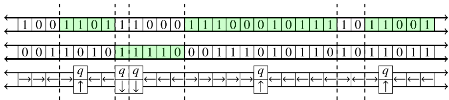
Figure 6. A finite word in A^* is divided into zones by the third layer. The dashed lines separate each zone and the colors indicate which tape is being pointed at by the arrow next to the state.
