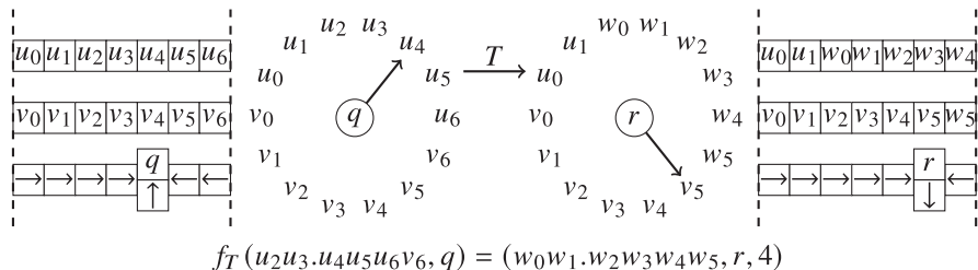
Figure 7. Every zone is wrapped around as a conveyor belt, where \phi(T) acts as if it were T seeing a periodic word.
