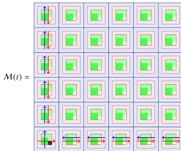
Figure 9. An example of macrotile \mathcal{M}(t) of side M = 6 . The red arrows represent the function \text{left}(t) = (1, 0) while the blue arrows represent \text{right}(t) = (0, 1) . The bottom left black square represents b_{5,1} = 1 .
