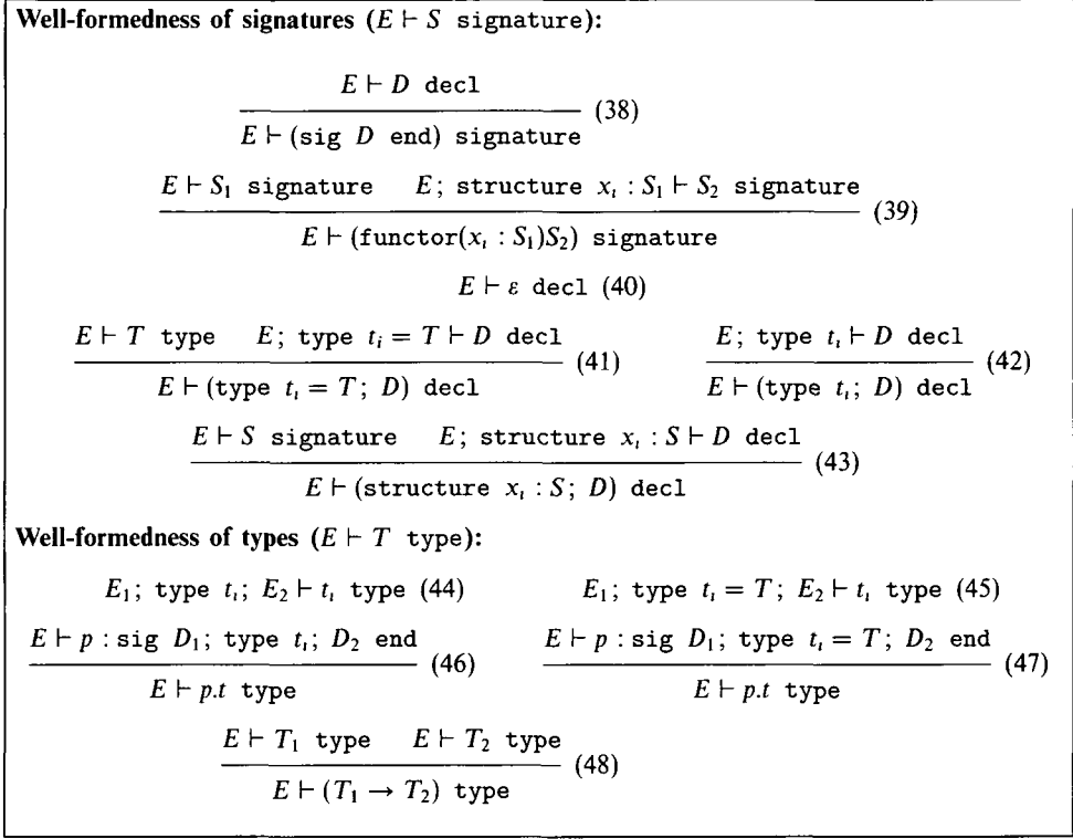
Fig. 3. Well-formedness judgements for the type system.
