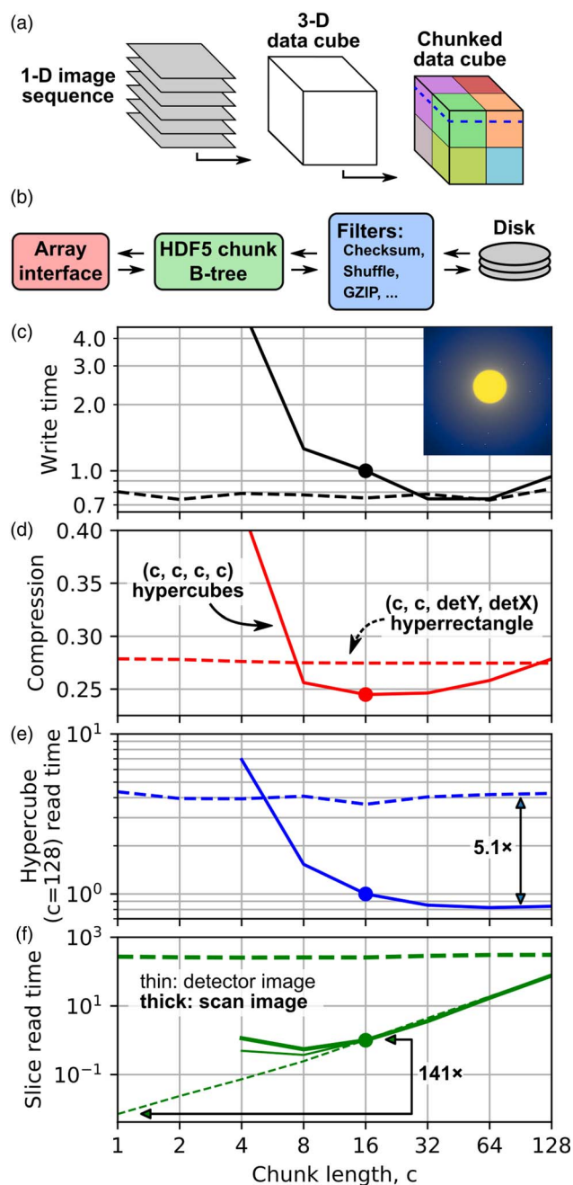
Fig. 6. (a) Example of potential dataset chunking for data from a 1D scan stored in an HDF5 file. (b) Data indexing sequence for chunked data. (c–f) HDF5 chunk performance metrics for the 256 \times 256 probe position STEM dataset from Figure 3 with a 256 \times 256 Medipix3 detector in a 12-bit mode. Level 4 GZIP compression was used. All panels show metrics for hypercube chunks (solid lines) and hyperrectangle chunks (dashed lines) with dimensions matching those of the detector (detY, detX). The inset in (c) shows a diffraction image on a logarithmic scale. The (e,f) read and (c) write times are the ratios of the values to those for the hypercube chunk length of 16 (marked by symbols). The compression ratios (d) are of the entire HDF5 file relative to only the raw Merlin binary file. The read times in (e) and (f) are those required to load a 128-sided hypercube or single slices of the dataset, respectively, into an in-memory NumPy array using h5py.
