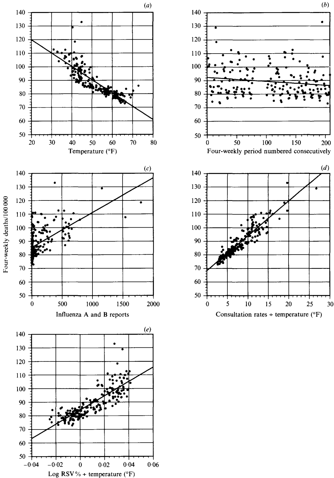
Fig. 2(a–e). Simple regression of y_1 , total 4-weekly deaths/100000, all causes excluding stillbirths, in England and Wales with: (a) x_{18} , weekly mean temperature (°F) recorded at London, Heathrow, (b) x_{10} , 4-weekly period numbered consecutively, (c) x_{13} , influenza A and B reports combined, (d) x_{20} = x_8 \div x_{18} , the interaction between consultation rates for aggregated acute upper respiratory tract infections and mean weekly temperature, (e) x_{21} = x_{16} \div x_{18} , the interaction between \log_{10} transformed 4-weekly RSV reports as a percentage of the total for the ‘winter’ and mean 4-weekly temperature (°F).
