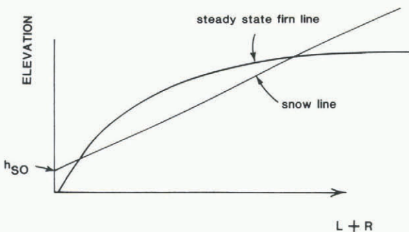
Fig.2. Schematic plot of ice-surface elevation at steady-state equilibrium firm line and snow-line elevation versus x = L+R .
