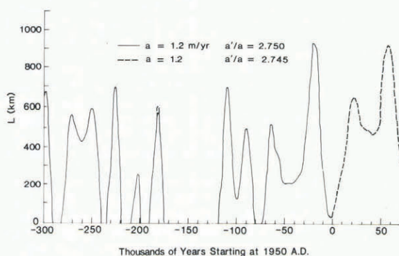
Fig.3. Half-width L of a Pleistocene ice sheet as a function of time and its prediction into the future for two slightly different accumulation rates (Weertman 1976).
