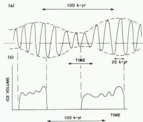
Fig.4. (a) A 20 ka signal with a modulated amplitude of 100 ka period used as forcing for an ice sheet. (b) A schematic history of ice-sheet volume change if ice-sheet growth is favored above dashed curve and destruction below it in (a) and a rapid (crash) destruction occurs under unusually large amplitudes.
