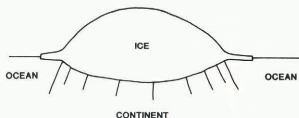
Fig.1. Cross-section of a two-dimensional ice sheet whose northern and southern borders terminate at the water's edge.
