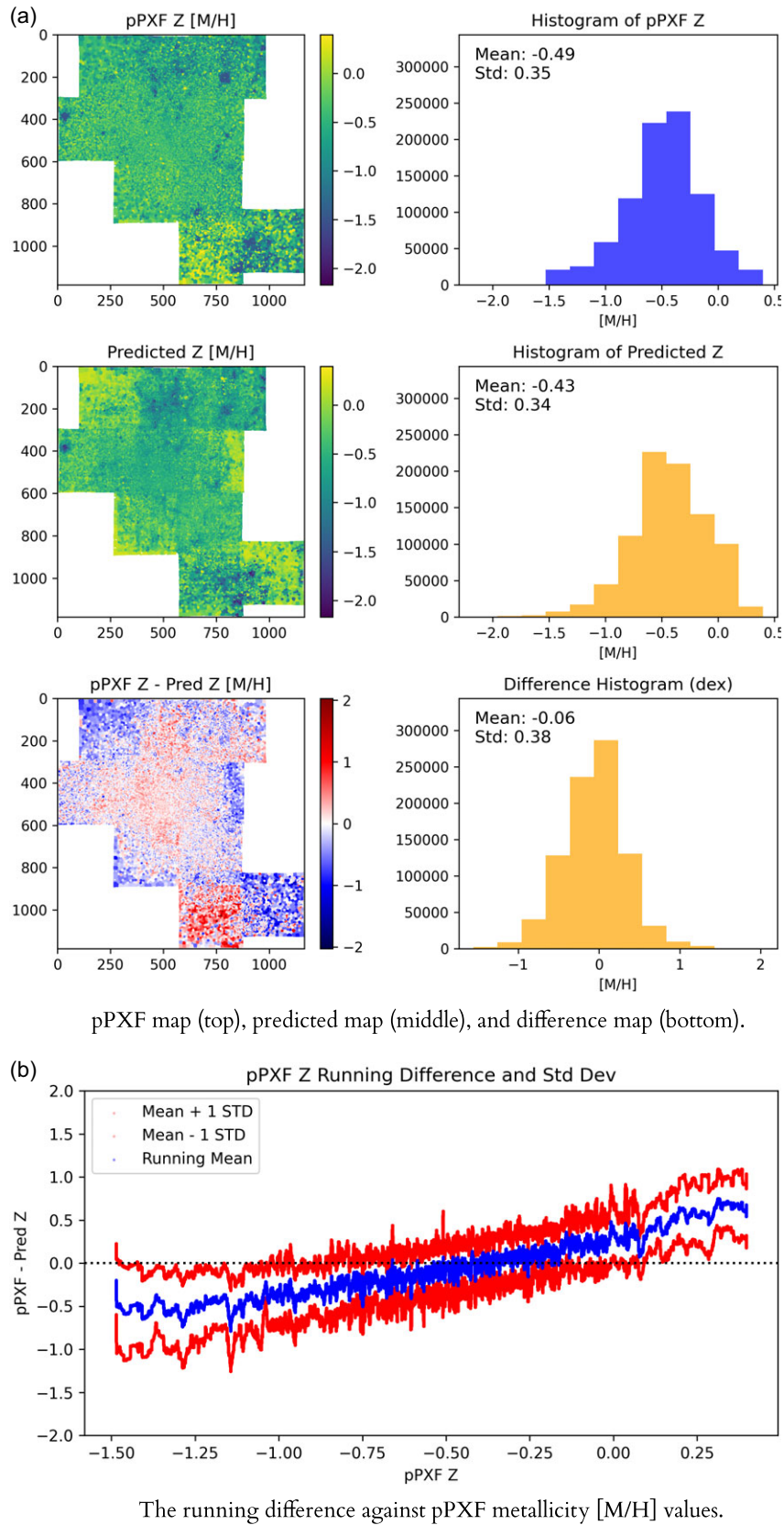
Figure 16. Metallicity maps and running difference for NGC5068.
