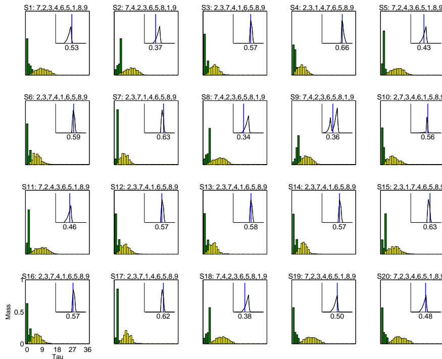
Figure 3: Performance of the two search models. Each panel corresponds to a subject, and their true cue search order is shown at the top. The histograms show the distribution of inferred search orders in terms of their tau distance from the true order. The green (dark) distribution is for the hierarchical model, and the yellow (light) distribution is for the non-hierarchical model. The inset shows the posterior distribution over the weight parameter in the hierarchical model, r
