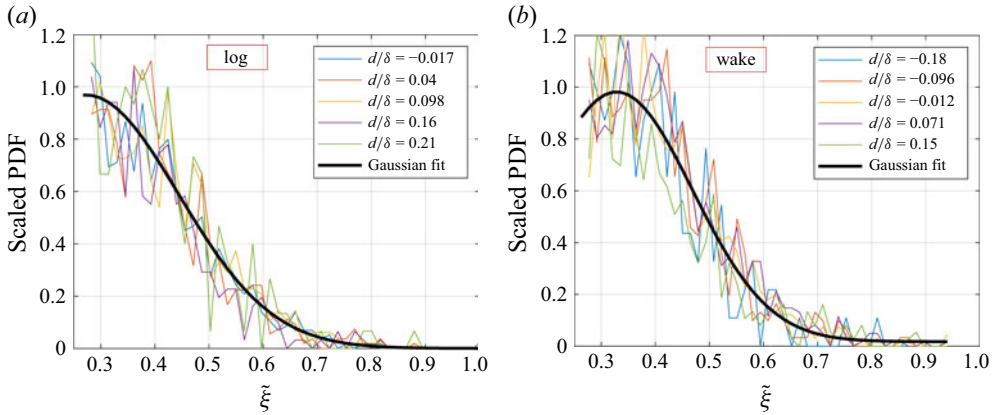
Figure 12. Normalised PDF of \tilde{\xi} at different wall-normal distances from the injection location for (a) log-injection and (b) wake-injection cases.
