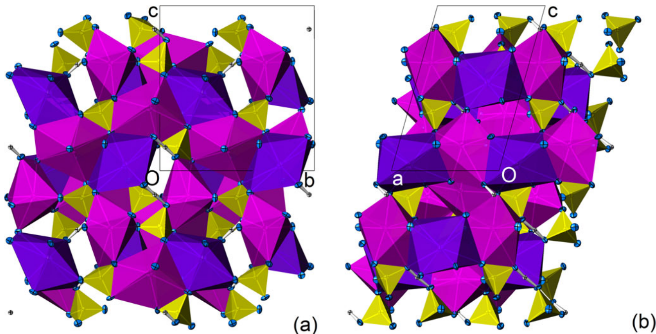
Figure 6. Crystal structure along [100]. Dark violet = K coordinations; magenta = Na coordinations; yellow = S coordinations; blue = O atoms; grey = H atoms. One unit cell indicated. Atomic displacement ellipsoids drawn at the 50% probability level.
