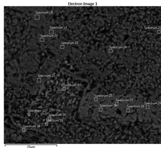
Figure 2. Back-scattered electron image of the sample where chemical composition of kristjánite was determined. Spots 18–20 + 22–24: kristjánite. Spots 25–29: mineral with tentative composition \text{K}_2\text{NaH}(\text{SO}_4)_2 .
