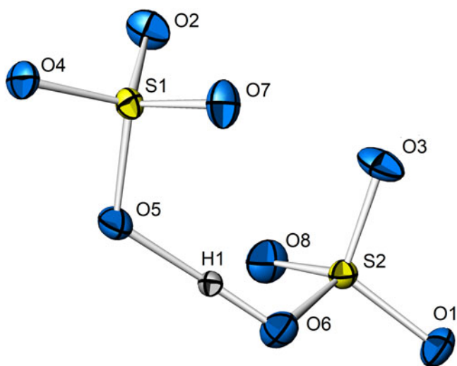
Figure 4. \text{SO}_4\text{-H-SO}_4 dimer. Atomic displacement ellipsoids drawn at the 50% probability level.
