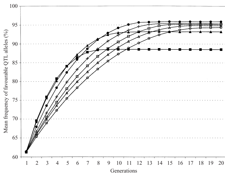
Fig. 2. Efficiency of truncation selection (MTS) for different selection intensities. Symbols indicate the number N' of individuals selected at each generation ( g > 0 ) among a total of 200: ■, 2; ▲, 4; ●, 10; +, 20; □, 30; △, 40; ○, 50. Abscissa, generation; ordinate, mean frequency of favourable QTL allele (%).
