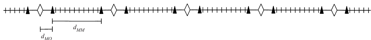
Fig. 1. Positions of QTLs and markers on a chromosome. \diamond , QTL; \blacktriangle , selected flanking marker; |, neutral marker.
