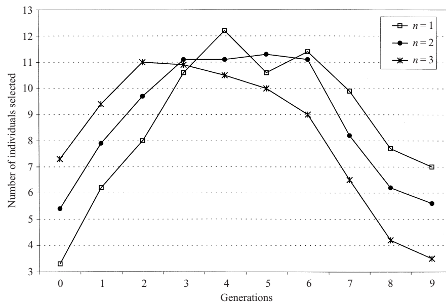
Fig. 3. Optimal intensity of truncation selection. Abscissa, generation; ordinate, number of individuals selected at each generation by the MTSC procedure for \theta_T = 1 and n_T values indicated by symbols: □, 1; ●, 2; ✱, 3.
