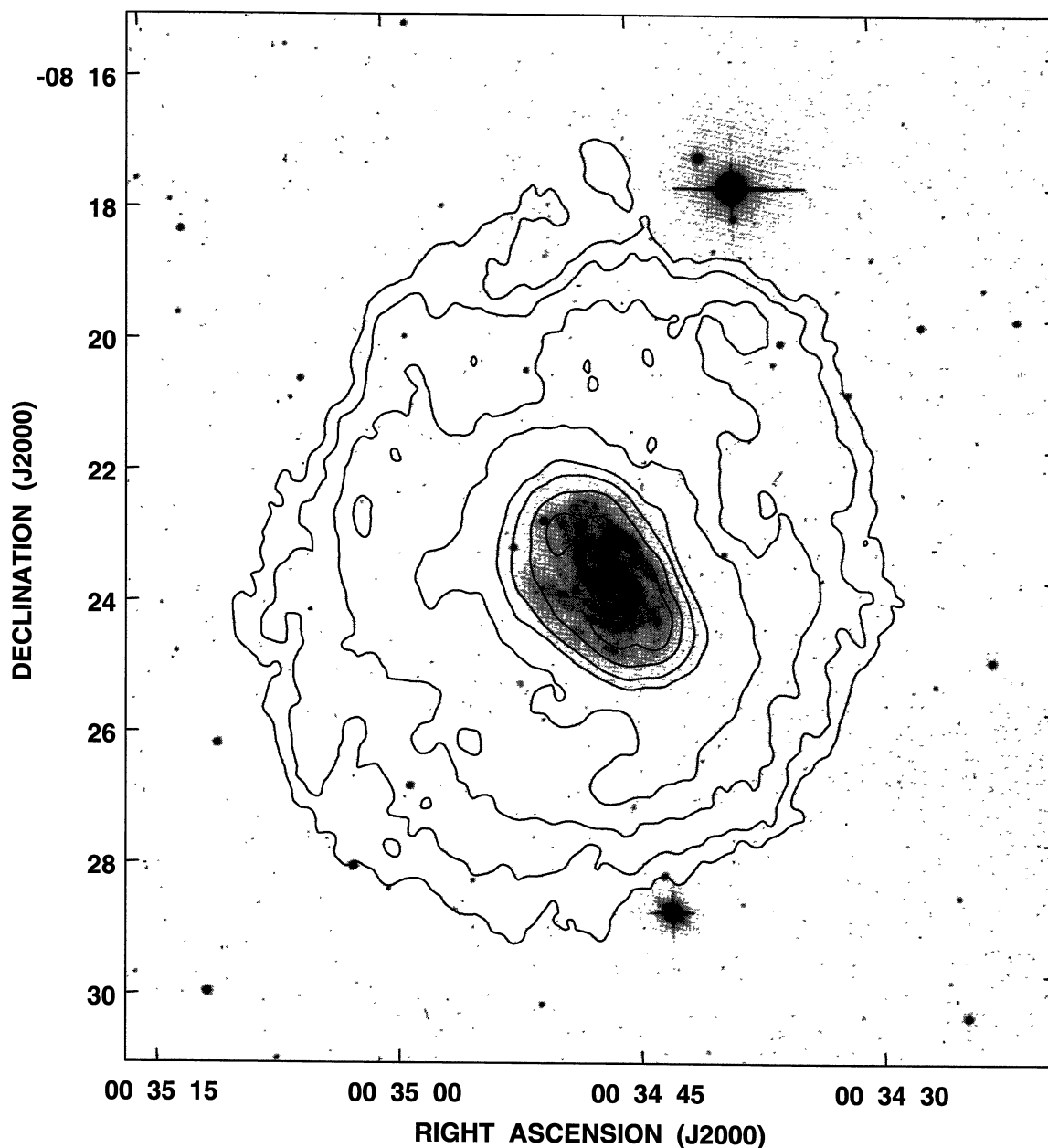
Figure 1 —Contours of H I column density overlaid on a B-band image of NGC 157. The contours correspond to (projected) column densities of 0.5, 1.0, 2.0, 3.5, 7.0, 10.0, 15.0 and 20.0 \times 10^{20} \text{ cm}^{-2} .
