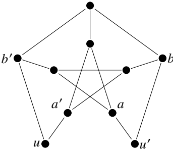
Figure 2. A Petersen star for r = 2 .
