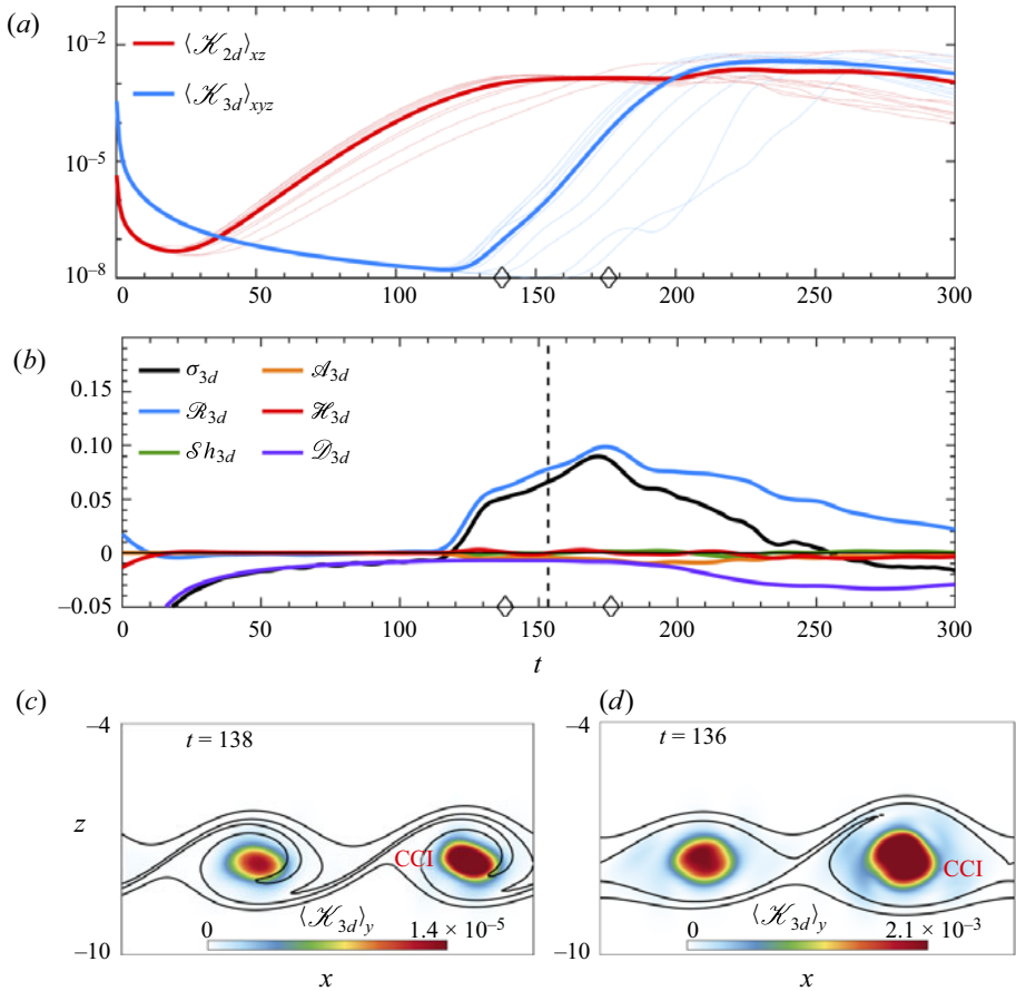
Figure 12. Similar to figure 11 but with the case d = 2.5 . Case #1 is selected for (c,d).
