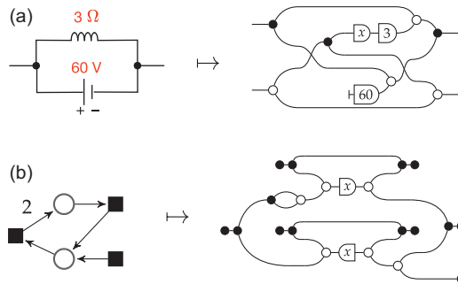
Figure 1.3 String diagrams representing the behaviour of an electrical circuit (a) and a Petri net (b). The abstract perspective offered by the diagrammatic approach reveals that seemingly very different phenomena may be captured via the same set of elementary components.
