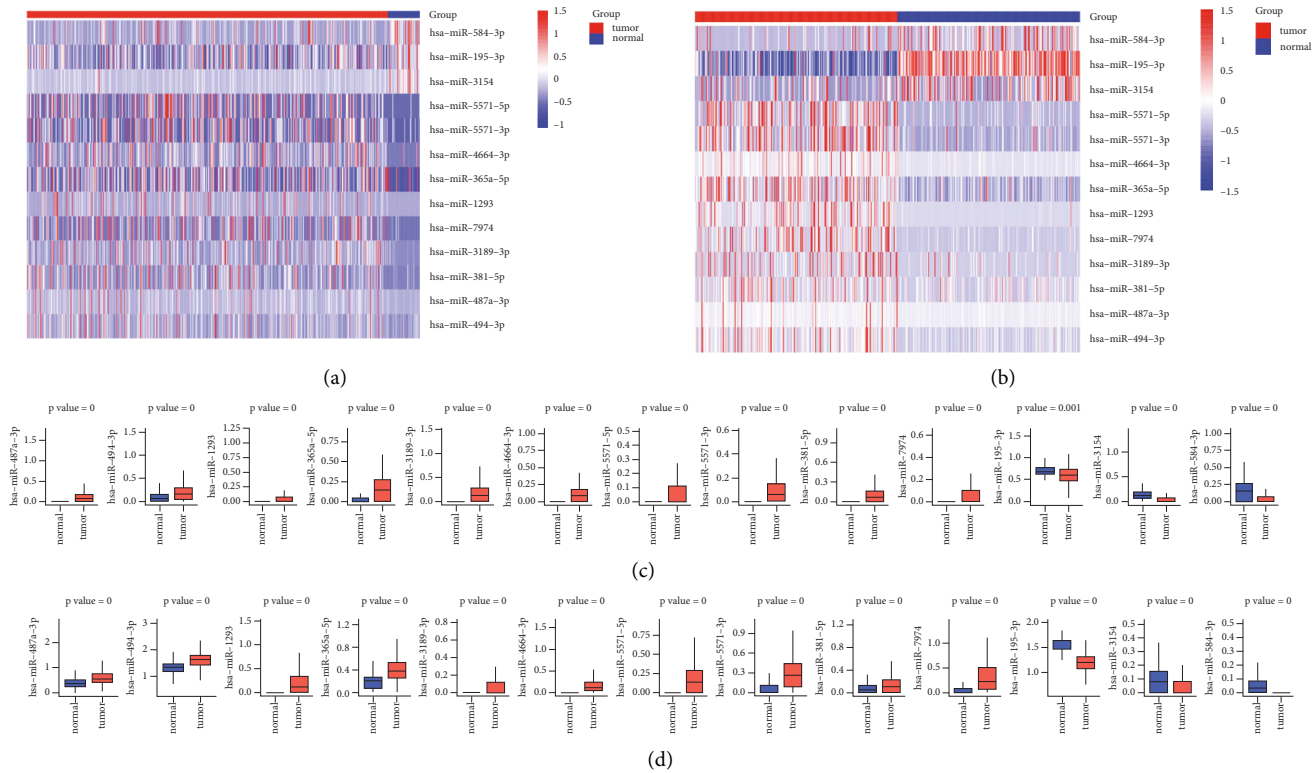
FIGURE 3: Univariate Cox regression analysis and Kaplan–Meier test on the selected differentially expressed miRNAs to further filter out eight miRNAs that are significantly related to OS. AB: 13 candidate microRNAs that are differentially expressed in tumors and normal tissues and are significantly related to OS ((a) expression heatmap in TCGA, (b) expression heatmap in CPTAC-3); CD: 13 candidate miRNAs in normal tissues (para-cancerous tissues) and tumor tissues. (c) Expression in the TCGA data set, (d) expression in the CAPAC-3 data set.
