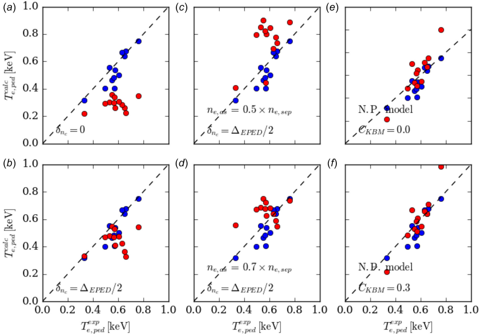
FIGURE 6. Predicted values of the pedestal electron temperature T_{e,\text{ped}}^{\text{calc}} vs experimental values T_{e,\text{ped}}^{\text{exp}} , with T_{e,\text{ped}}^{\text{calc}} calculated using the standard EPED model (•) and from each of the various EPED based pedestal models (•) corresponding to the same model cases as in figure 5 (a–f) above, each for all of the 2.0 MA pulses from the isotope mass and fuelling rate scans in table 1.
