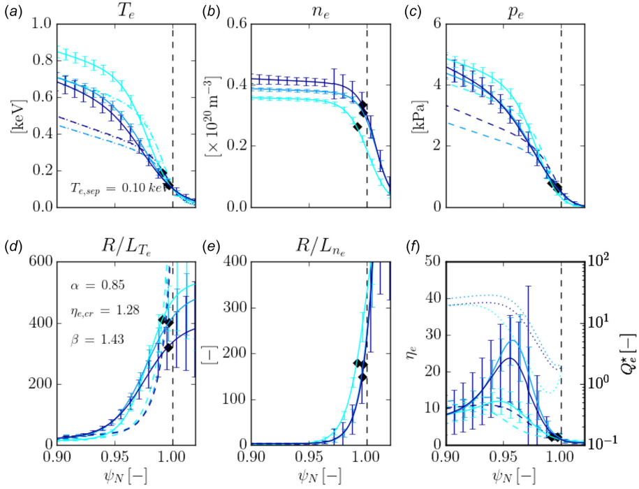
FIGURE 3. Pedestal profiles for the three 2 MA JET-Be/W H-mode deuterium pulses ( A_{\text{eff}} = 2 ) from table 1 no. 96202 (cyan), no. 96208 (mid-blue) and no. 96201 (dark-blue) with gas fuelling rates of \Gamma_{\text{gas}} \sim 0.74, 1.7 and 2.7 \times 10^{22} \text{ es}^{-1} , respectively, with the plotted quantities as defined in figure 1.
