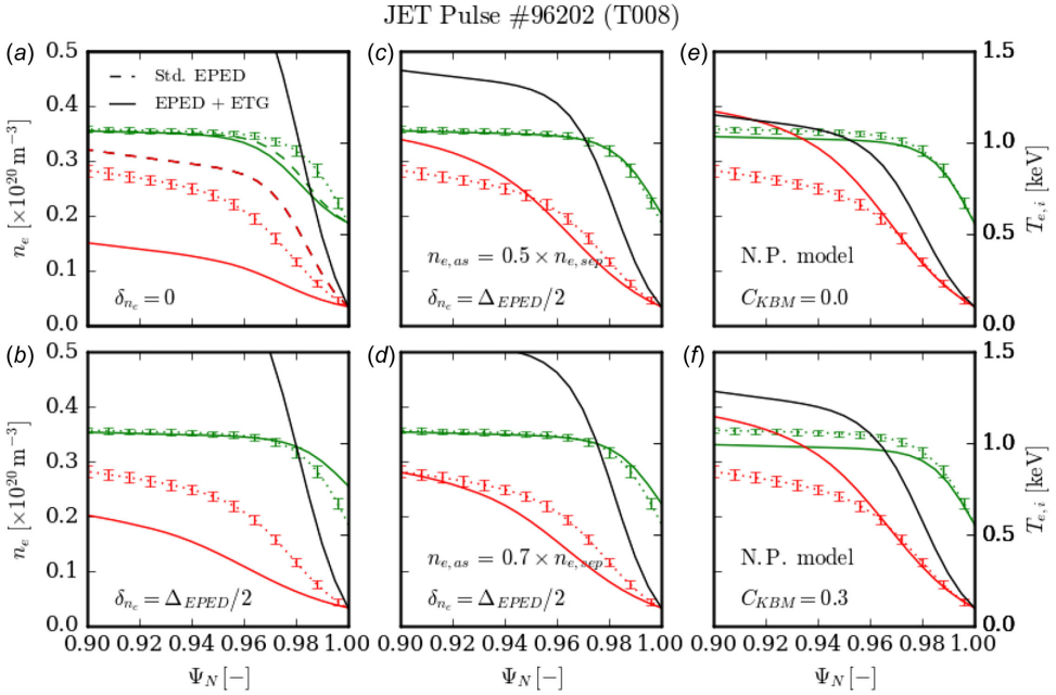
FIGURE 5. Pedestal profiles for the D pulse no. 96202 at the low fuelling rate of \Gamma_{gas} \sim 0.74 \times 10^{22} \text{ es}^{-1} showing n_e (green), T_e (red) and T_i (black) vs normalised poloidal flux \psi_N from various EPED based models. Experimental profile fits are shown by the ‘dotted’ lines with the error bars. Profiles are shown in (a) calculated using standard EPED (‘dashed’ lines) and from the combined ETG + EPED model (M2) (‘solid’ lines). In (b–d) the n_e profile is shifted outwards by \delta n_e = \Delta_p/2 , with T_e calculated using the ETG model; in (c) the n_e profile asymptotes to 0.5 \times n_{e,sep} outside the separatrix; in (d) the n_e profile asymptotes instead to 0.7 \times n_{e,sep} . In (e, f), the n_e profile is calculated using the DP model of Saarelma et al. (2023), the T_e profile is calculated using the ETG model and T_i is determined for consistency with the EPED prediction of p_{tot} ; in (e) with coefficient C_{KBM} = 0 and in (d) with C_{KBM} = 0.3 .
