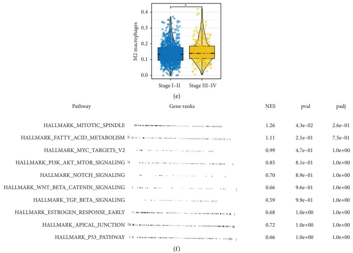
FIGURE 1: Exploration of M2 macrophages in lung cancer. (a) Quantification of M2 macrophages through the CIBERSORT algorithm in lung cancer; (b) KM survival curves of patients with high and low M2 macrophage infiltration; (c)–(e) M2 macrophage infiltration difference in patients with different clinical features, including T stage, N stage, and clinical stage, ns = P > 0.05 , * = P < 0.05 , *** = P < 0.001 ; (f) biological enrichment of M2 macrophages based on the hallmark gene set.
