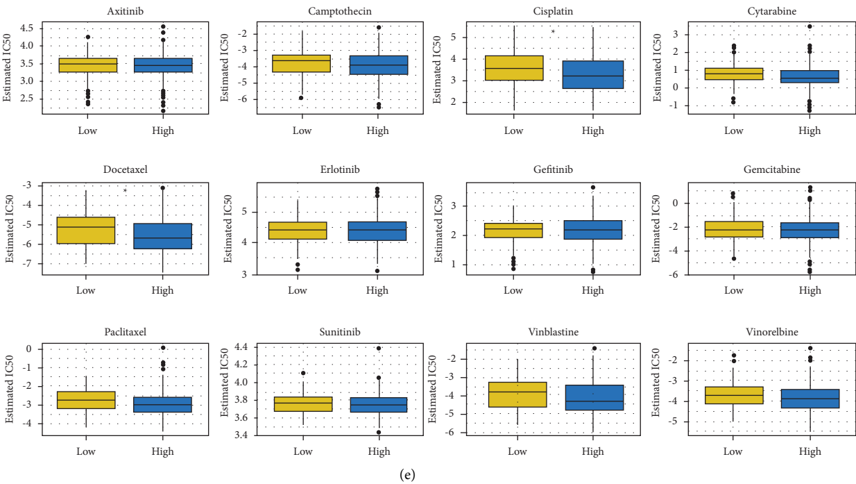
FIGURE 5: Immunotherapy and chemotherapy sensitivity. (a) The TIDE algorithm was used to evaluate the response of lung cancer patients on immunotherapy; (b) correlation between risk score and TIDE score; (c and d) low-risk patients had a lower TIDE score and a high percentage of immunotherapy responders, * = P < 0.05 ; (e) chemotherapy sensitivity difference between high- and low-risk patients, * = P < 0.05 .
