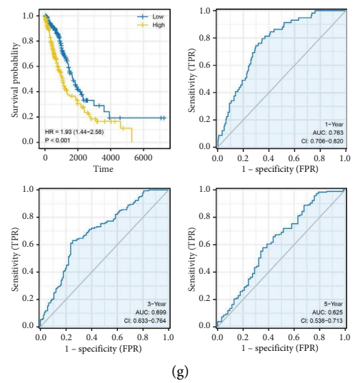
FIGURE 3: Construction and validation of prognosis signature. (a and b) LASSO regression of input genes; (c) multivariate Cox regression based on the genes identified by LASSO regression; (d) overview of the risk score in the training cohort; (e) KM survival and ROC curve of high- and low-risk patients in the training cohort; (f) overview of the risk score in the validation cohort; (g) KM survival and ROC curve of high- and low-risk patients in the validation cohort.
