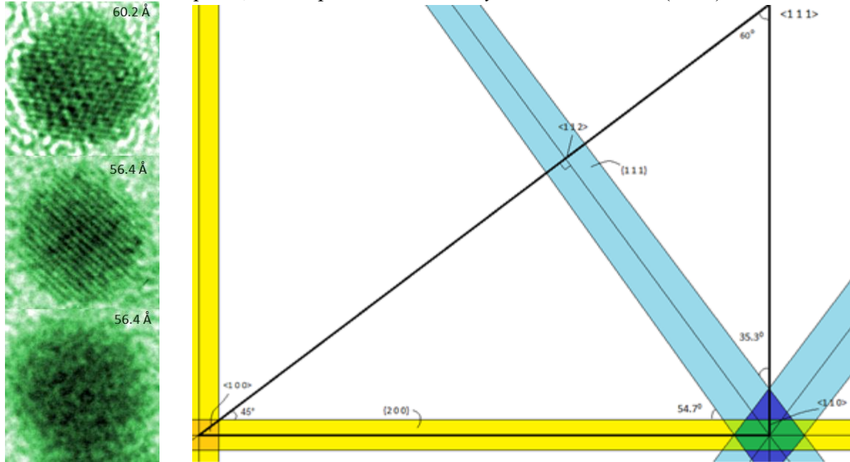
Figure 1. (left) Examples of cross, single, and no fringes shown. Fieldwidths listed on each image. Figure 2. (right) 2-D schematic of asymmetric unit in FCC map.
