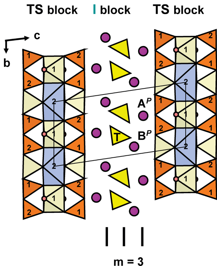
Figure 4. The crystal structure of ferroinnelite projected onto (100). Legend as in Fig. 3; Ba atoms at the A^P and B^P sites are shown as raspberry-coloured spheres, TO_4 ( T = S, P ) tetrahedra are yellow. The three vertical lines show the positions of the cation layers ( m = 3 ) in the I block.
