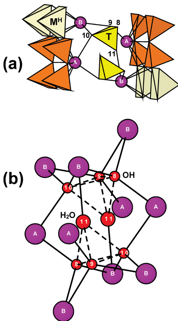
Figure 5. Details of short-range order of anions in the I block for ferroinnelite: (a) linkage of Ba atoms (at the ^{[9]}A^P and ^{[11]}B^P sites) and TO_4 tetrahedra where T tetrahedra are fully occupied by S and P; (b) linkage of Ba atoms at the A^P and B^P sites via OH [O(8,9,10)] and H_2O groups [O11] where T sites are vacant. Legend as in Fig. 4; Ba atoms at the A^P and B^P sites are shown as raspberry-coloured spheres and labelled A and B, respectively. Anions in the I block are (a) not shown where they are O atoms which coordinate T sites occupied by S and P and (b) shown as small red OH and large red H_2O spheres where T sites are vacant. Thin black lines in (a) and (b) show Ba–O bonds; dashed lines in (b) show possible hydrogen bonds.
