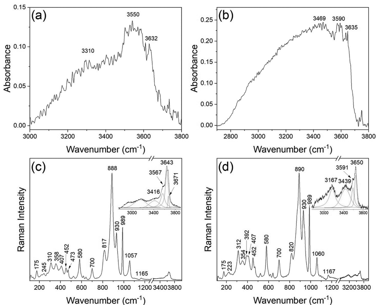
Figure 2. Infrared spectra of (a) ferroinnelite (crystal 9530_2) and (b) holotype innelite (crystal 81801_1) in the principal OH-stretching region; Raman spectra of (c) ferroinnelite and (d) holotype innelite from ~100 to 4000 \text{cm}^{-1} ; the OH stretching range is shown in the inset where the pattern decomposition is given as a guide to the eye.
