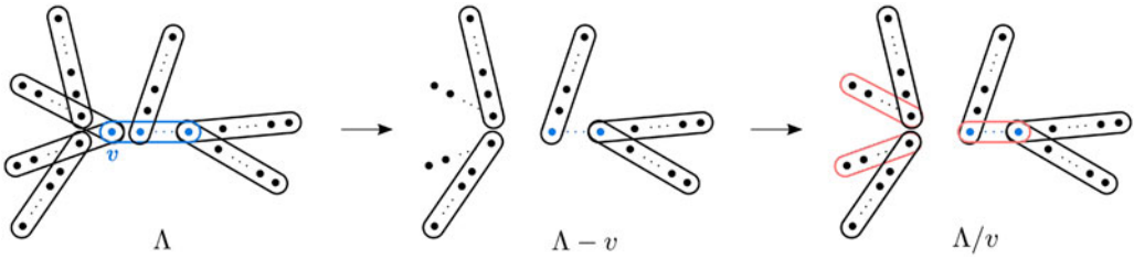
Figure 2. Obtaining \Lambda/v from \Lambda if v is not in a 2-edge.
