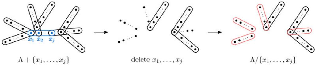
Figure 3. Obtaining \Lambda / \{x_1, \dots, x_j\} from \Lambda + \{x_1, \dots, x_j\} .
