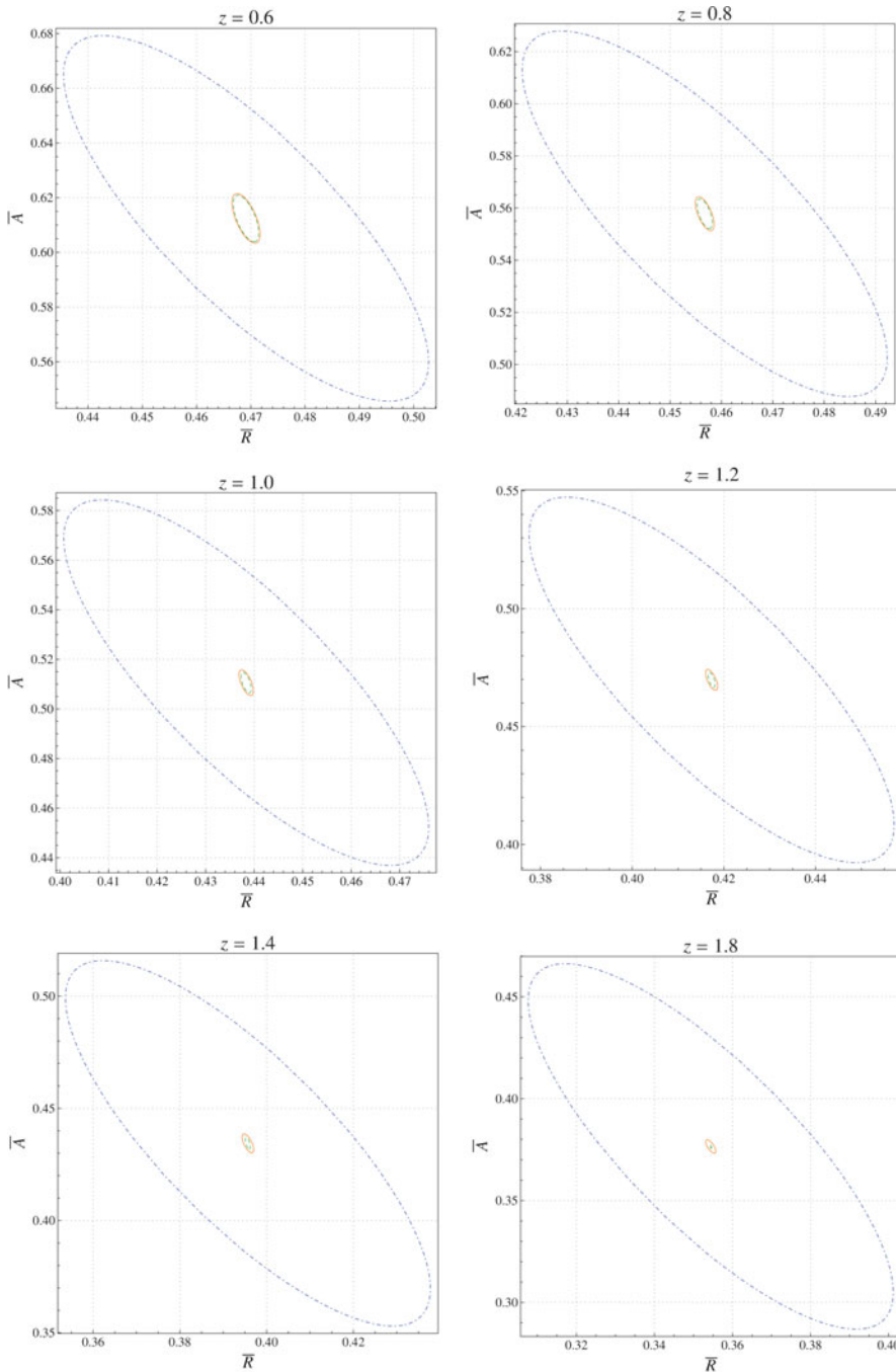
Figure 1. Confidence contours for \bar{A} and \bar{R} in the three cases: Solid line V_{\text{eff}} , dot dashed line V_{\text{eff}} \approx V_{\text{survey}} , and dashed line V_{\text{eff}} \approx P(k, \mu)^2 .
