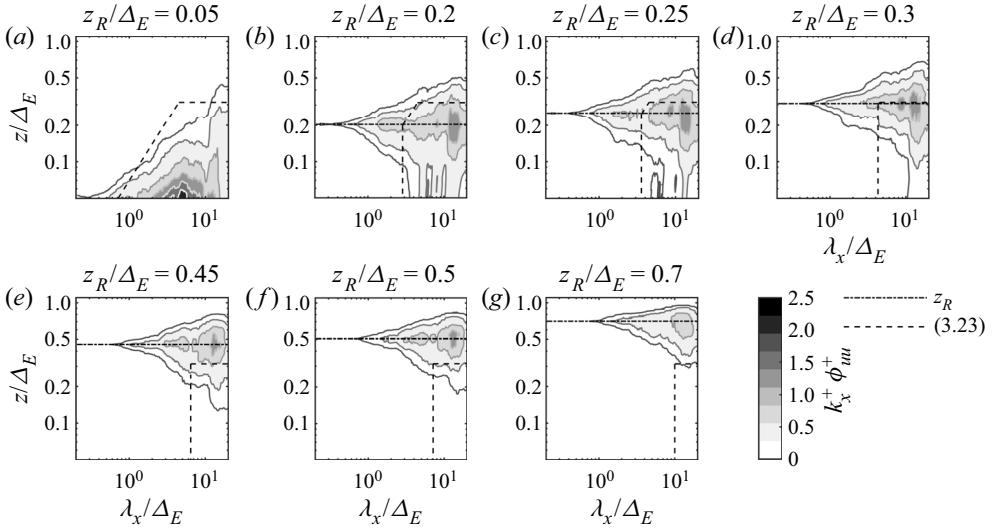
Figure 12. Coherent portion of the streamwise velocity energy spectra calculated for different reference heights, z_R .
