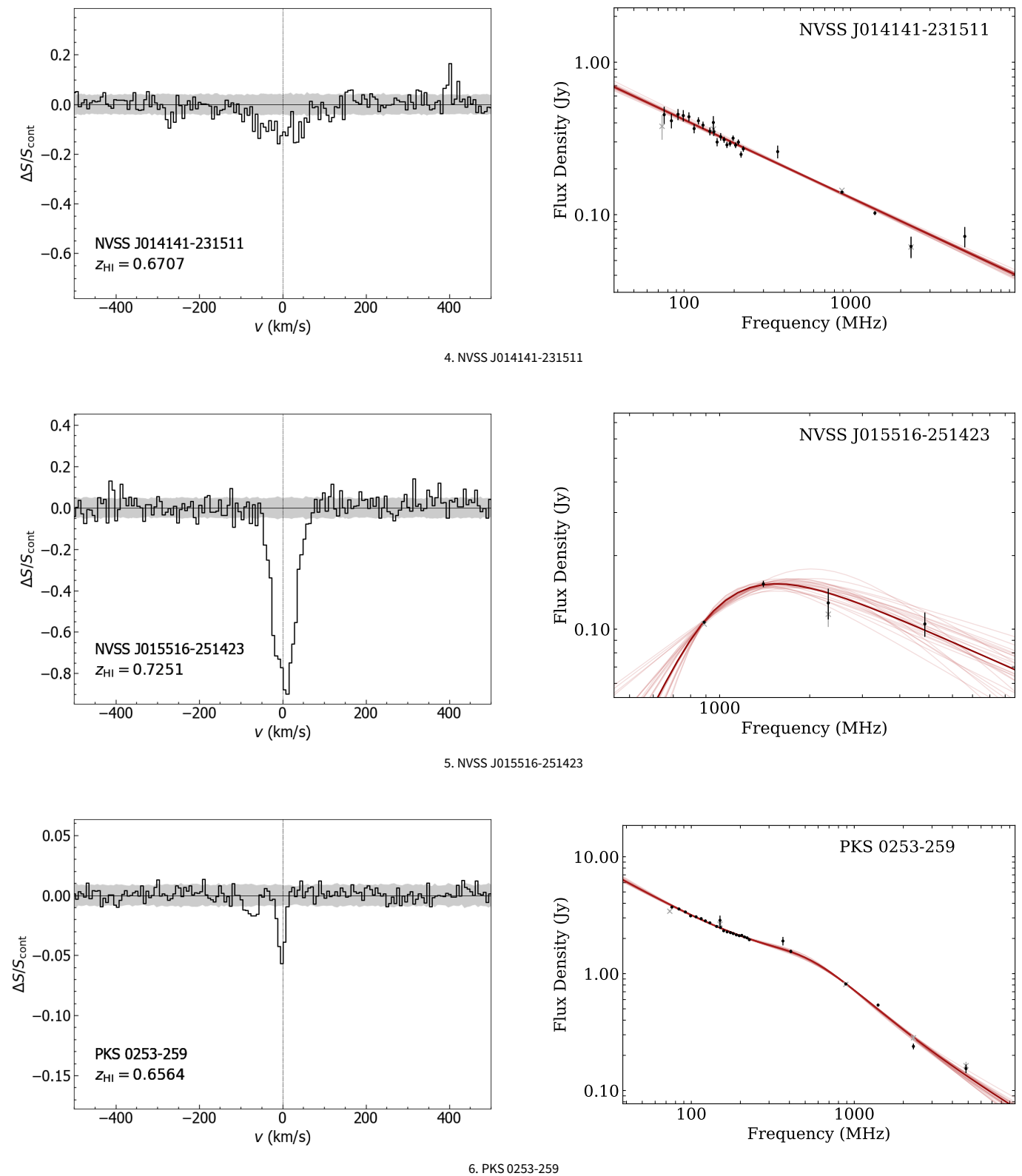
Figure A4. (continued) Spectral-line profiles and radio SED fits for: 4. NVSS J014141-231511 (top), 5. NVSS J015516-251423 (middle), and 6. PKS 0253-259 (bottom).
