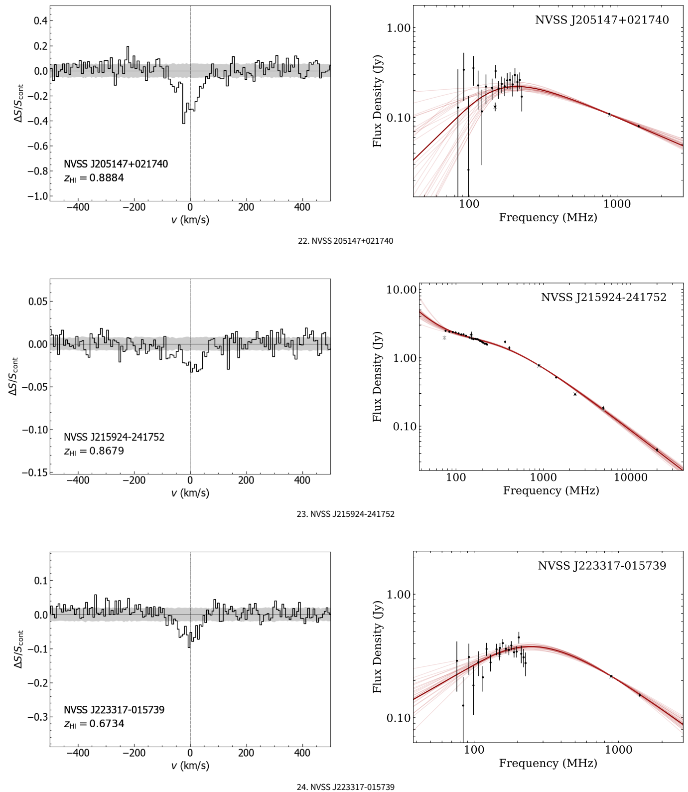
Figure A4. (continued) Spectral-line profiles and radio SED fits for: 22. NVSS 205147+021740 (top), 23. NVSS J215924-241752 (middle), and 24. NVSS J223317-015739 (bottom).
