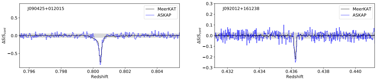
Figure 18. Spectra of FLASH detections observed with MeerKAT (black line) overlaid with the ASKAP spectrum (blue). The grey band denotes the 5-\sigma noise level calculated from the MeerKAT spectra.
