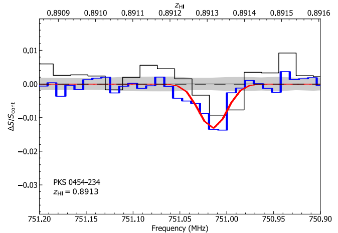
Figure A3. Line profile of PKS 0454–23. Blue and red lines are from Gupta et al. (2012) . Black is from our observation (SBID 34547_1a). The grey shaded region is the 1\sigma level of the rms spectral-line noise.
