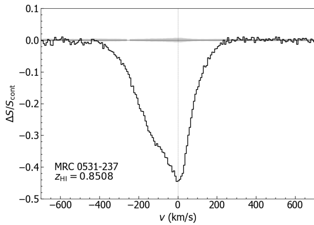
10. MRC 0531-237
