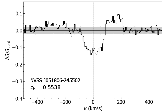
9. NVSS J051806-245502
