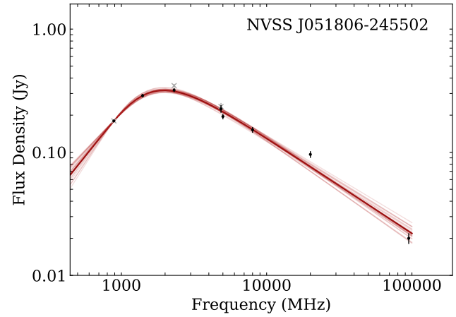
Figure A4. (continued) Spectral-line profiles and radio SED fits for: 7. PKS 0405-280 (top), 8. SUMSS J045501-423858 (middle), and 9. NVSS J051806-245502 (bottom).
