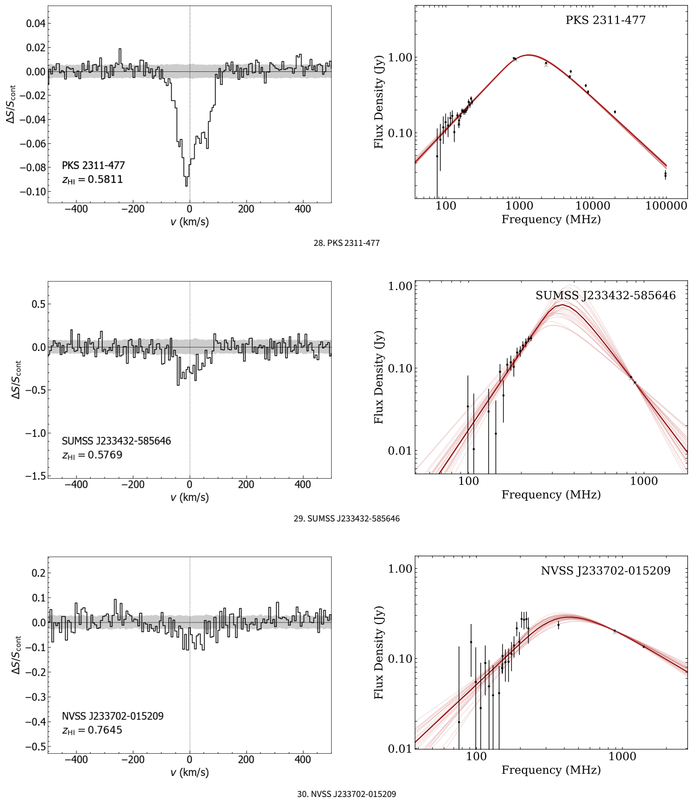
Figure A4. (continued) Spectral-line profiles and radio SED fits for: 28. PKS 2311-477 (top), 29. SUMSS J233432-585646 (middle), and 30. NVSS J233702-015209 (bottom).
