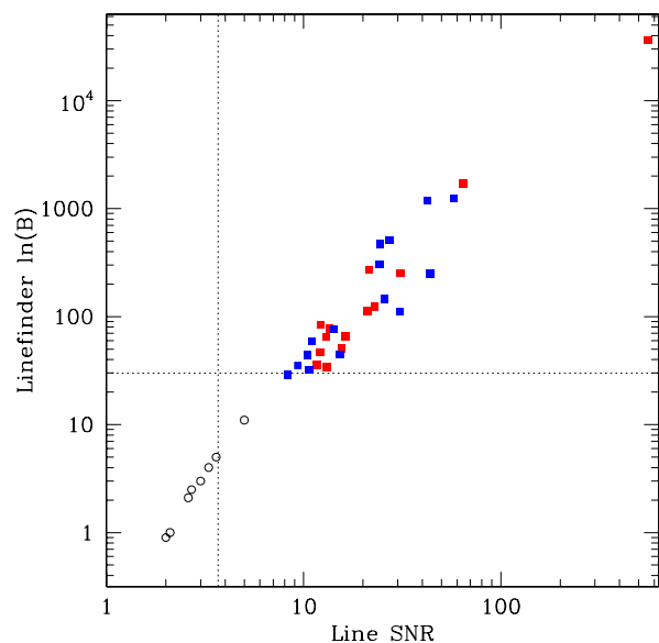
Figure A2. As in Figure A1 , except that the SNR values plotted are now integrated over the whole line, assuming a gaussian profile. In this plot, black open circles at lower \ln(B) show values tabulated by Benneke & Seager (2013) and the vertical dotted line corresponds to the 3.6\sigma value considered by Trotta (2008) to be ‘strong’ evidence.
