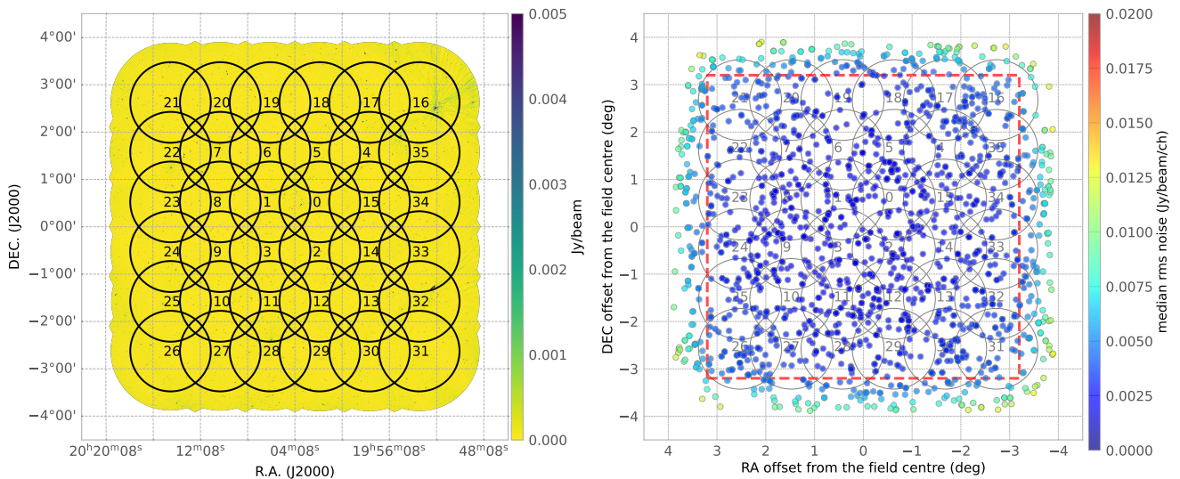
Figure 3. FLASH field of view and noise properties: (left) a FLASH continuum image showing the position of the 36 ASKAP beams in the square_6x6 footprint used to form the image, (right) measurements of spectral-line noise for extracted spectra in a 6-hour Pilot 1 observation (SBID 13293), showing that the noise is roughly uniform within the central red dashed square, covering 6.4 deg x 6.4 deg on the sky (total area 40.9 deg 2 ).
