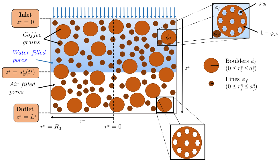
Figure 1. A cartoon of the bed geometry. The liquid is injected at the inlet, located at z^* = 0 and exits the bed through the outlet at z^* = L^* . During infiltration, the wetting front is located at z^* = s_w^*(t^*) . The local volume fractions of the liquid, fines and boulders are given by \phi_l , \phi_f and \phi_b respectively. The volume fraction of pore space within a boulder is given by \phi_{lb} .
