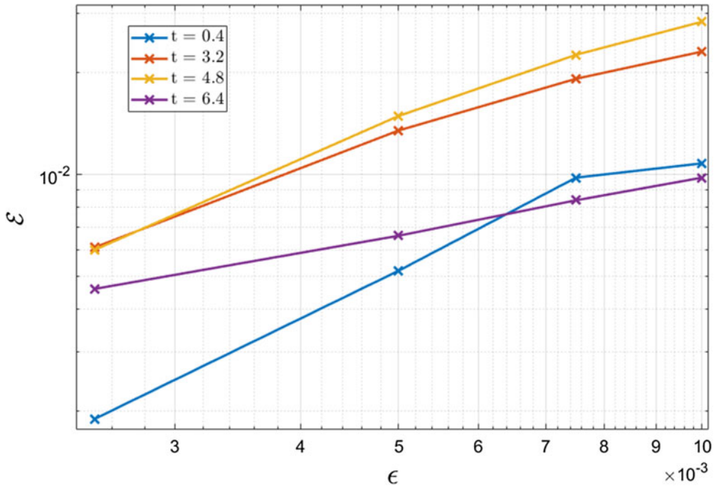
Figure 5. An error analysis of the results in Figure 3. The error measure is defined as \mathcal{E}(t) = \sum_{i=1}^{i=n} (c_l^{num}|_{x=x_i} - c_l^{asy}|_{x=x_i})^2 / n in which x_i are the locations of the mesh points; and the superscripts are used to distinguish the numerical solution of the full model ('num') from the numerical solution of the asymptotically reduced model ('asy').
