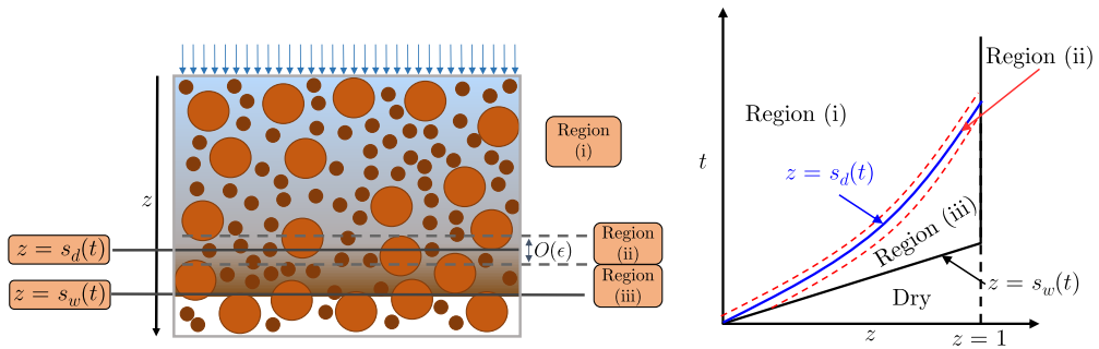
Figure 2. Schematics to illustrate the asymptotic structure of the problem. The left panel shows a snapshot of the different regions of the bed arising in the asymptotic analysis along with the moving boundaries s_d(t) and s_w(t) . The right panel shows the location of these moving boundaries evolving in the z - t plane. The wetting front, s_w(t) , is represented by the solid black line. Region (iii) is located adjacent to the wetting front, region (i) is adjacent to the inlet. The saturation interface represented by the solid blue line and located at z = s_d(t) , is surrounded by a narrow region (ii).
