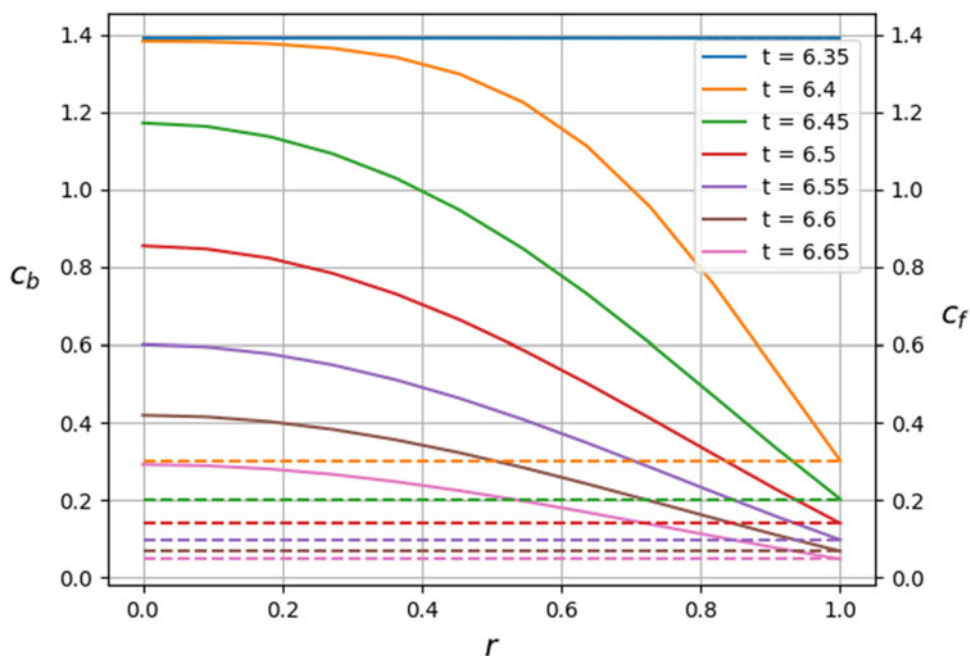
Figure 7. Concentration profiles inside the grains located at z = 1 . Solid lines show profiles in the interior of the boulders at the listed times. Dashed lines show constant concentration across the interior of the fines at corresponding times.
