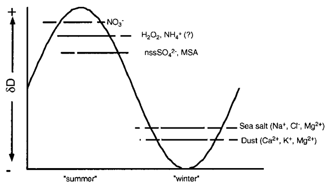
Fig. 6. Summary of seasonal input timing at Siple Dome, relative to an idealized \delta D curve (after Whitlow and others, 1992). Solid lines indicate when maximum concentrations frequently occur, and dashed extensions represent the range where peaks are sometimes noted.
