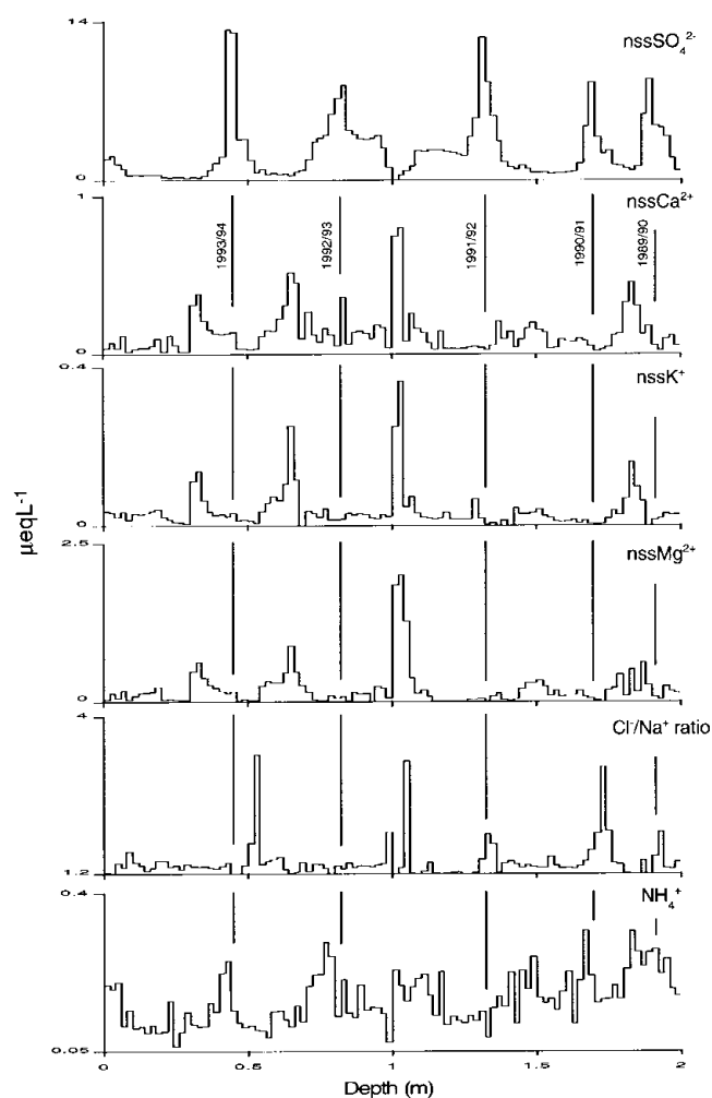
Fig. 5. Comparison of nssSO_4^{2-} , nssCa^{2+} , nssK^+ and nssMg^{2+} concentrations, Cl/Na^+ ratios and NH_4^+ concentrations in pit 94-I. Pit 94-I is presented here because it is located at the site of a 150 m ice core (Kreutz and others, 1997a). The temporal pattern of variability demonstrated for these species in pit 94-I is consistent in all other pits.
